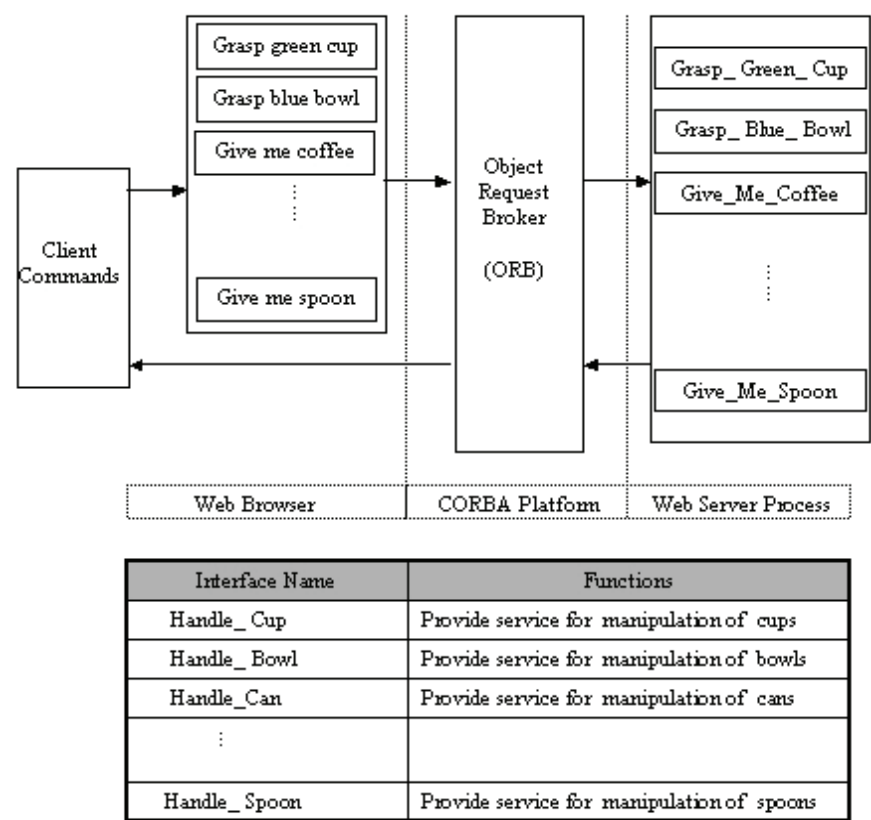
Fig. 4. Robot control server and its interface.
