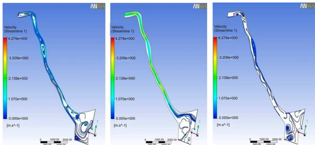
Fig. 5. Lines of transient currents in the Rio Matapi: a) low tide at t = 1\text{h} , b) end of the ebb at t = 5.5\text{h} , c) reversal of the tide at t = 6\text{h} .
