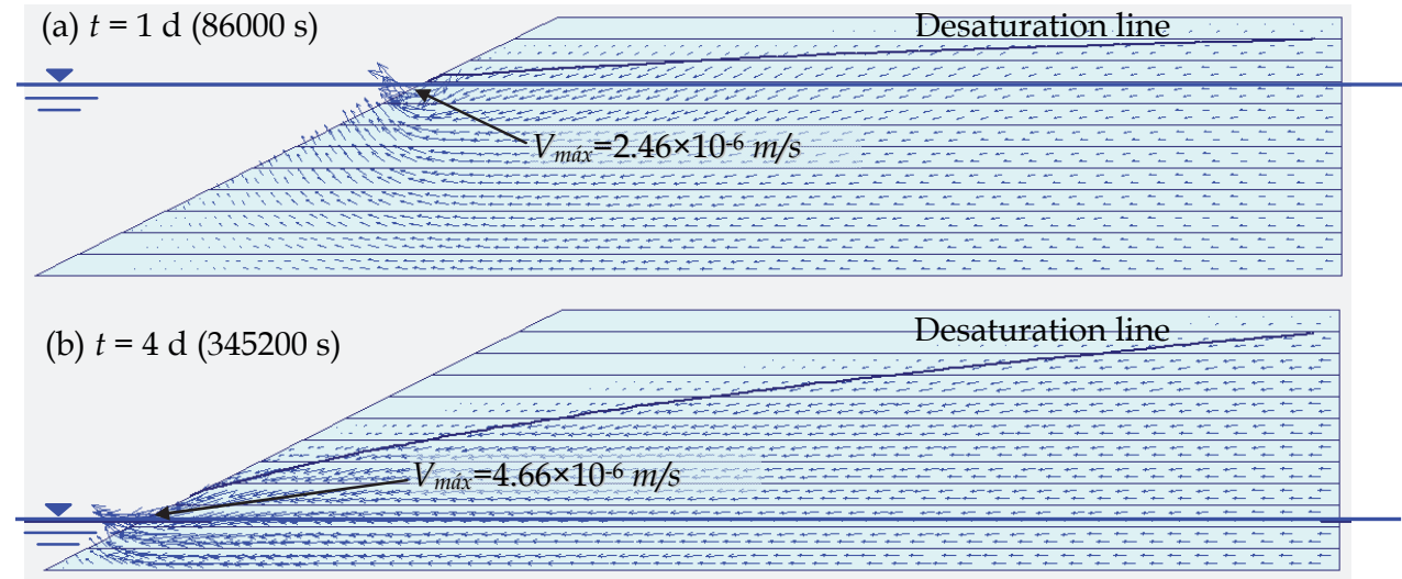
Fig. 16. Velocity vectors (magnitude) for two different time intervals during rapid drawdown (Auvinet & Lopez-Acosta, 2010)
