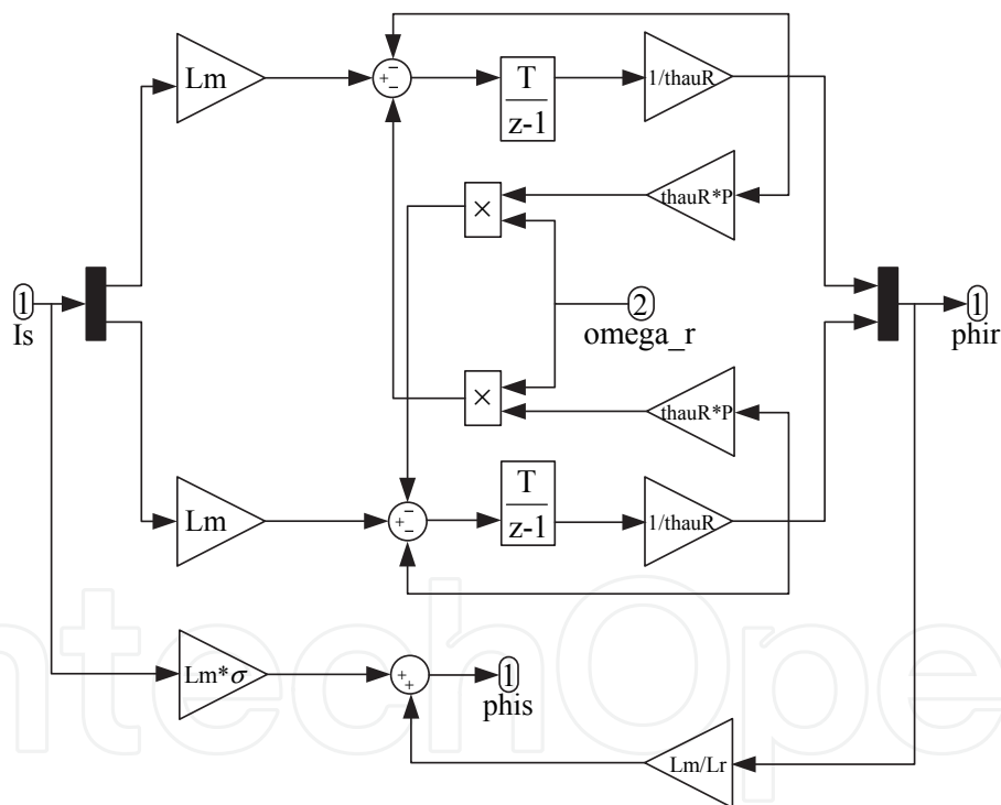
Fig. 10. Fluxes observers implemented in Matlab/Simulink/dSPACE environment
