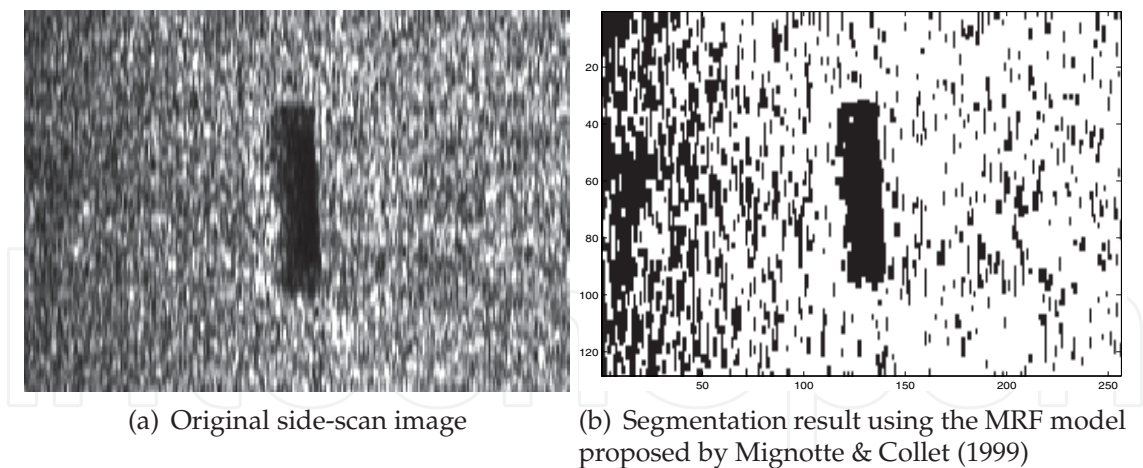
Fig. 7. MRF segmentation
