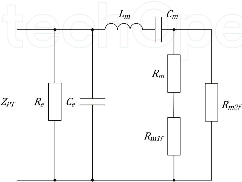
Fig. 7. Non-linear electrical model of piezoelectric ceramic transducer
