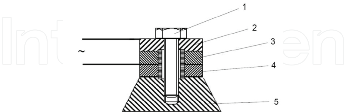
Fig. 2. Construction of sandwich type piezoelectric ceramic transducer; 1 – screw or pin settings (gripping), transmitter, 2, 5 – blocks of metal (eg. aluminum, iron, brass), 3, 4 – piezoelectric ceramic plates (cylindrical, annular)
