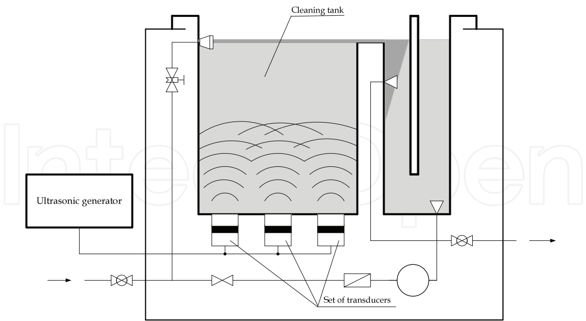
Fig. 1. Ultrasonic cleaning system
