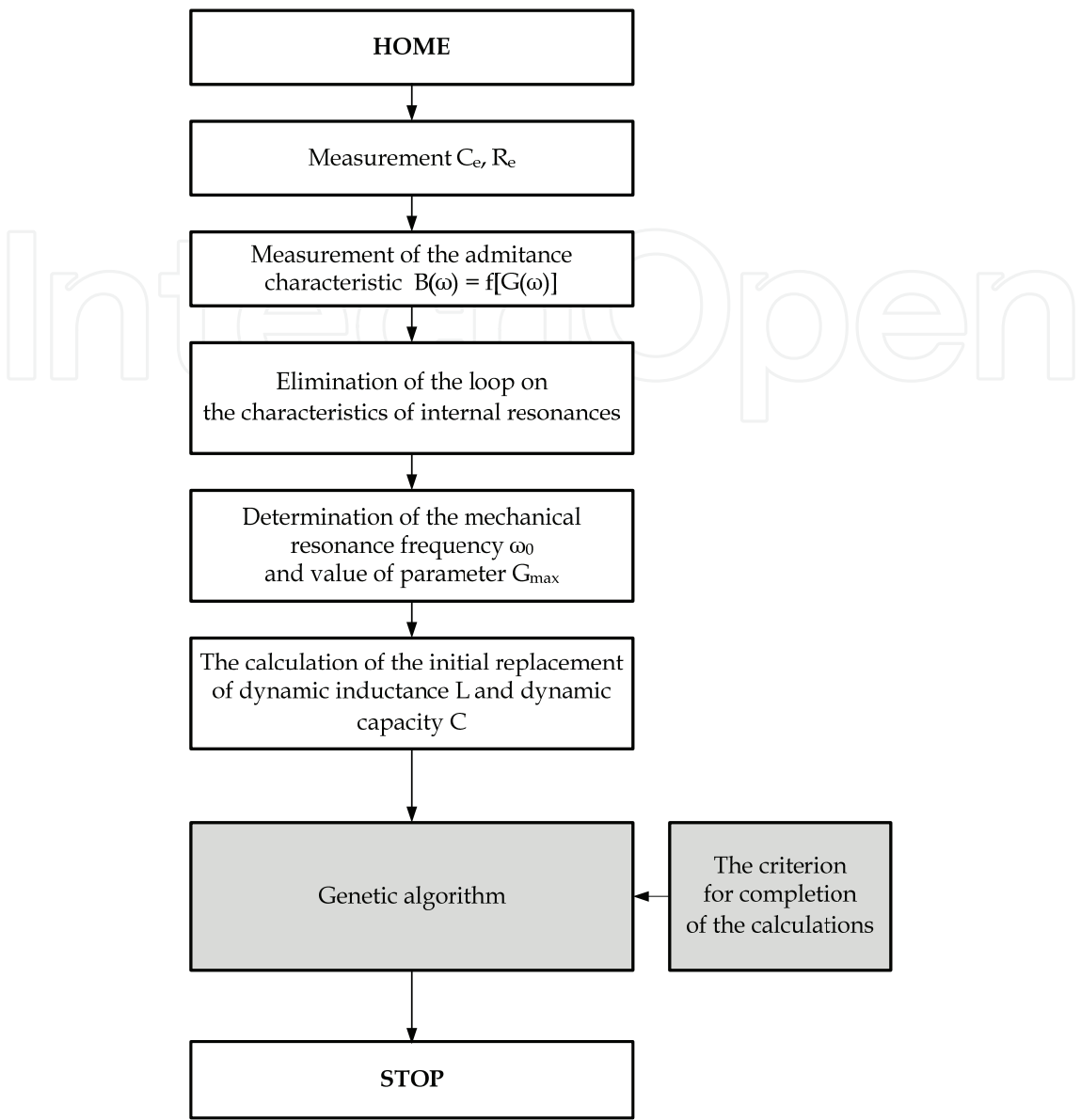
Fig. 12. Algorithm for parameter identification of dynamic model of the branch of electrical power ultrasonic transducer
