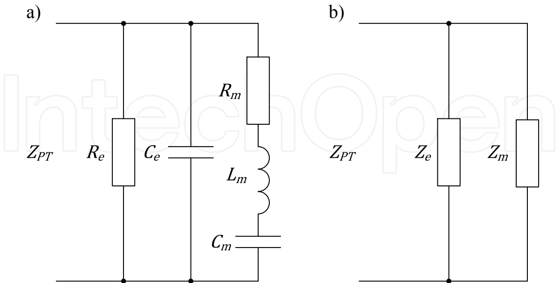
Fig. 5. Linear, a replacement wiring diagram piezoelectric ceramic transducer, Z_{PT} - Electrical impedance of the transmitter: a) a detailed diagram, b) the distribution of the branch of electrical and mechanical
