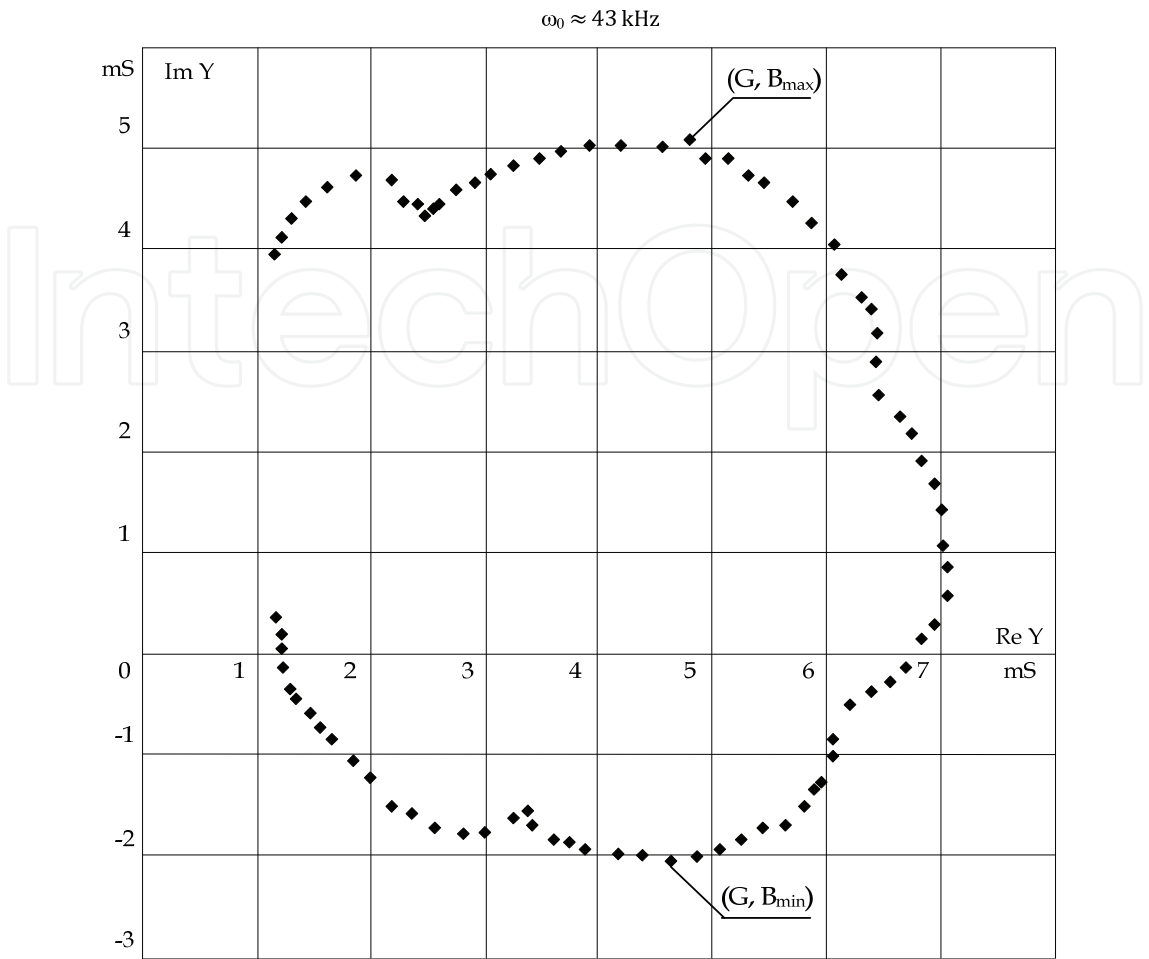
Fig. 10. The actual characteristics of the transducer after eliminating resonances fringe The set of coordinates of the actual approximation characteristics transducer (Fig. 9) is a database for further calculations.
