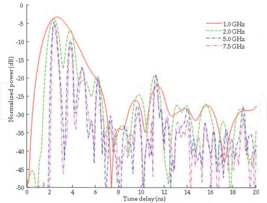
Fig. 7. A detail of normalized power delay profiles at d = 0.78 m for different bandwidths.
