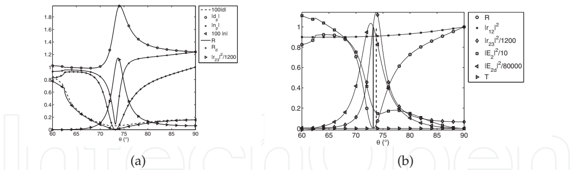
Fig. 3. (a) Reflected intensity R = |r/n|^2 , and |n_d/d|^2 (Eqs. 9,10) and numerators and denominators: |n| , |d| , |n_p| and |d_p| . (b) Plot of the amplitude of fields inside the gold layer |E_2| and |E_{2d}| and of the reflection coefficient on each interface (Glass/Gold: r_{12} and Gold/Water: r_{23} . All plot are functions of the angle of incidence \theta , and are computed for n_1 = 1.5 , n_2(\lambda_0 = 670 \text{ nm}) = 0.137 + 3.797i , n_3 = 1.33 , e = 50 \text{ nm} .
