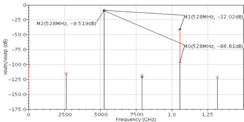
Fig. 17. Simulation result of the MUX with and without the dummy pairs
