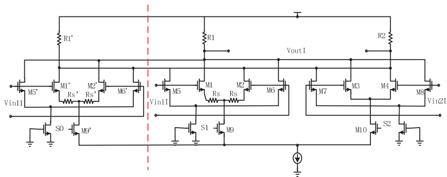
Fig. 16. Schematic of the multiplexer
