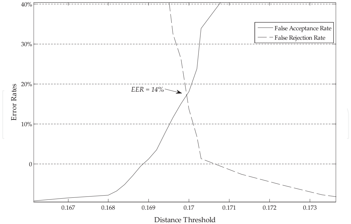
Fig. 5. False Acceptance and Rejection Rates after personalization of the thresholds.
