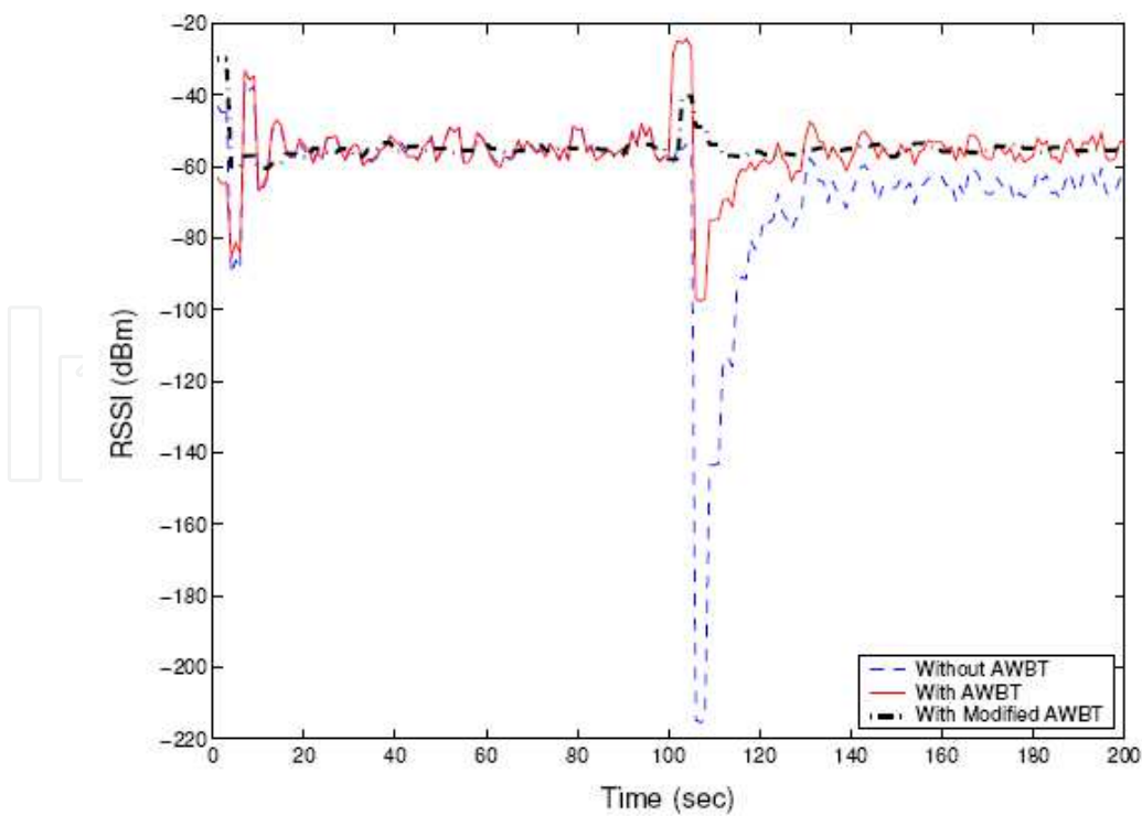
Fig. 26. Modified AWBT performance ignoring saturation constraints and where handoff occurs at 100 (sec)
