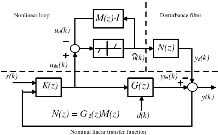
Fig. 11. Equivalent representation WPAW conditioning technique.
