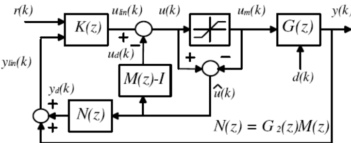
Fig. 10. Weston Postlethwaite Anti-Windup conditioning technique.
