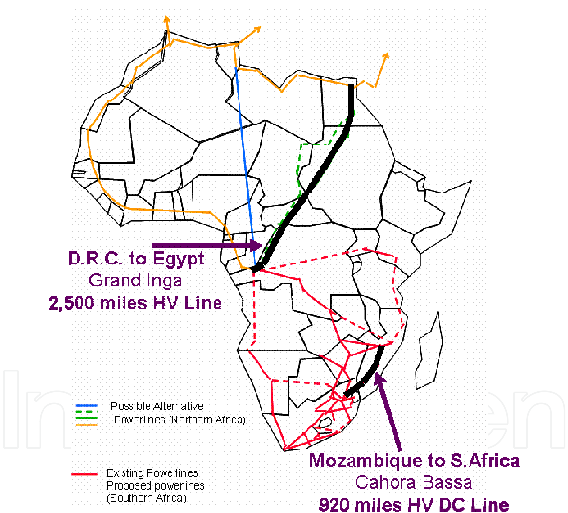
Figure 19.4. Long-Term Transmission Planning in Africa
