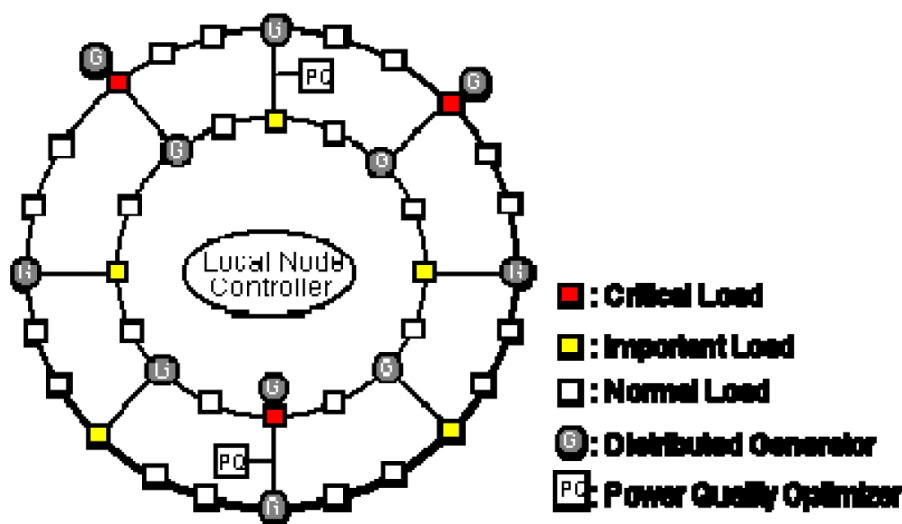
Figure 19.15. Formation of Double-Ring Local Node
