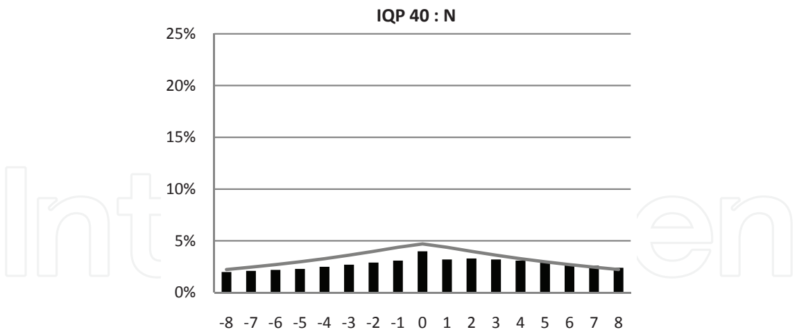
Fig. 7. The new method for correlation noise estimation is more accurate for coarse quantization (i.e. low rates).
