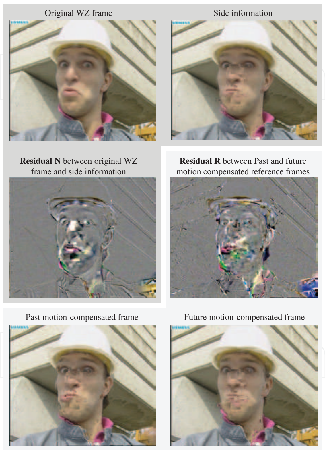
Fig. 4. Correlation noise N compared to the motion compensated residual R (fine quantization, intra quantization parameter of 10 is employed for the reference frames).
