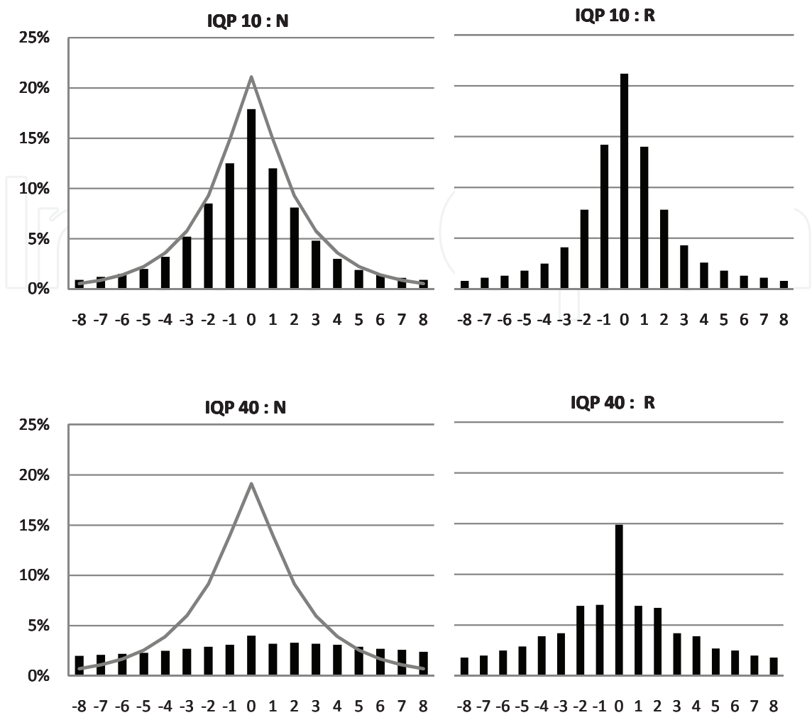
Fig. 6. Measured distribution of N and R , for the luma DC component of Foreman, for different quantization levels (H.264/AVC intra quantization parameter given). The average estimated distribution of N is drawn on top. Clearly, we can see that while the estimated noise is close to the true noise for fine quantization (IQP 10), there is a significant mismatch for coarse quantization (IQP 40).
