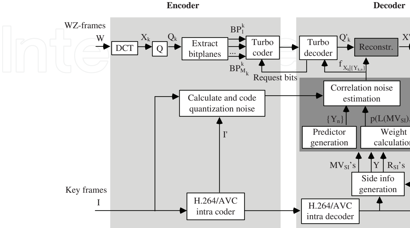
Fig. 10. The DVC codec featuring a correlation model that compensates for quantization noise and m
