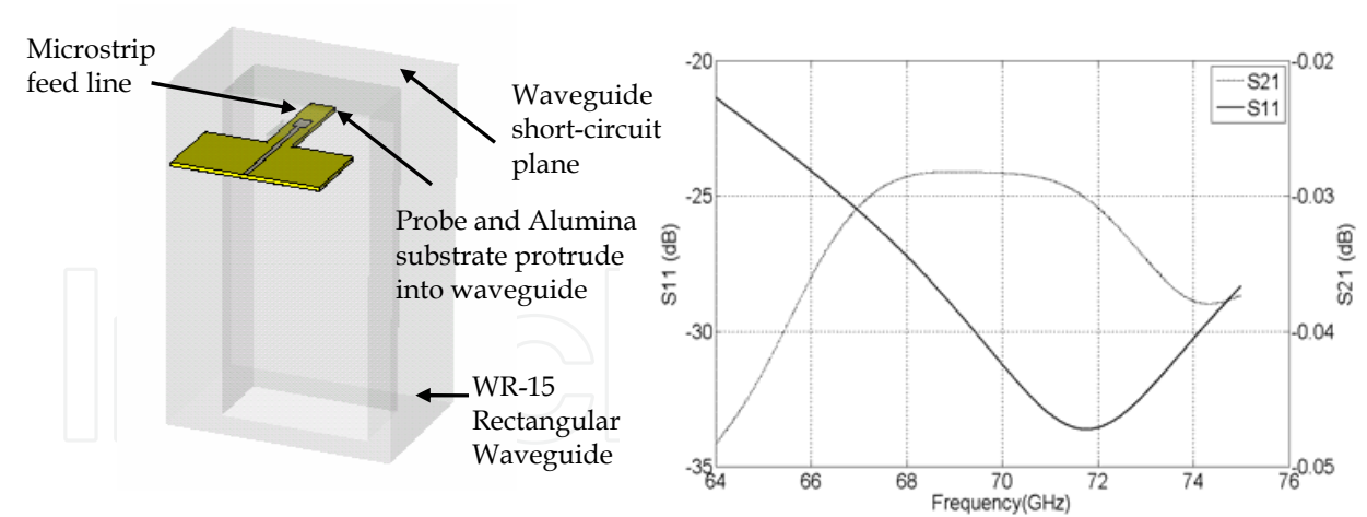
Fig. 13. a) Waveguide-to-microstrip transition b) Predicted reflection and transmission coefficients of the waveguide-to-microstrip transition
