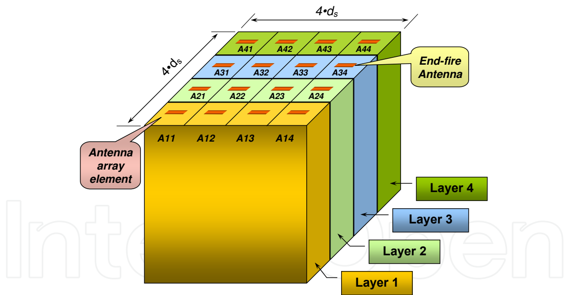
Fig. 4. Configuration of a 4x4 element square lattice sub-array. Each “layer” represents a four-element sub-module integrated on a common printed circuit board
