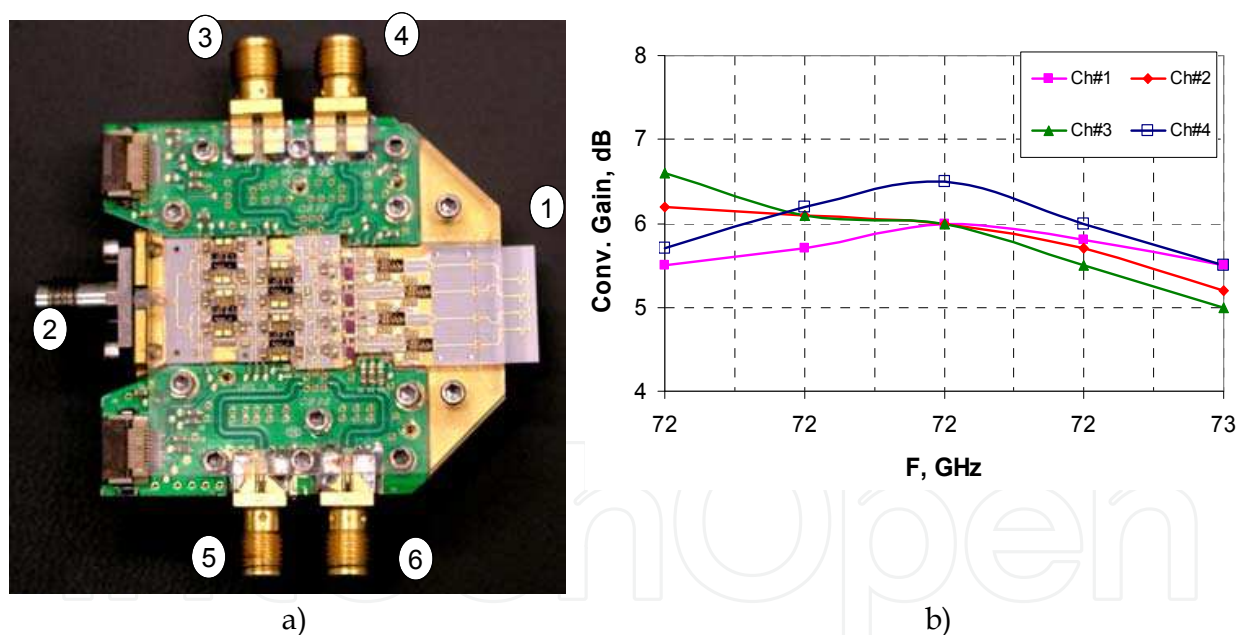
Fig. 7. a) Photograph of the RF module assembly where: 1 is the antenna array; 2 is the LO input; 3-6 are IF outputs; b) Typical measured conversion gain (RF to IF1) for each channel
