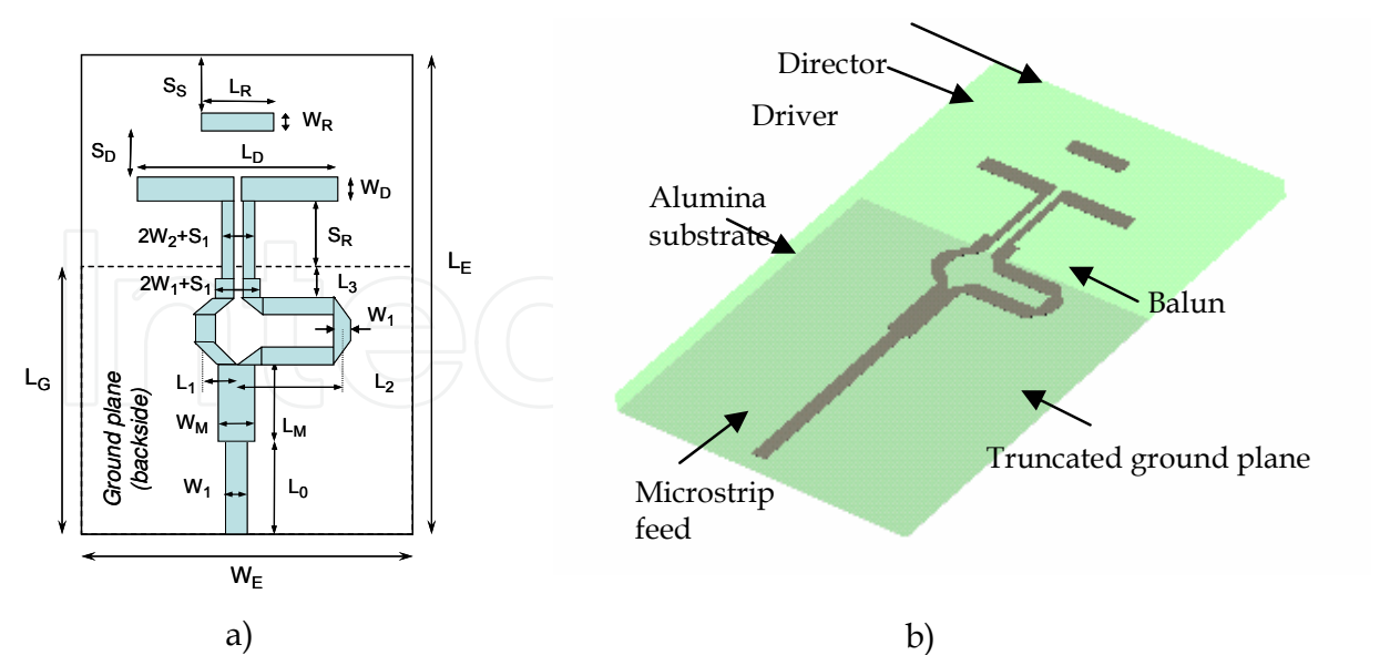
Fig. 8. Schematic of the quasi-Yagi antenna array element. L_E=3 , W_E=2.5 , W_1=0.12 , L_0=0.45 , L_G=1.54 , L_M=0.54 , W_M=0.205 , L_1=0.22 , L_2=0.7 , L_3=0.1 , S_1=0.06 , W_2=0.06 , L_D=1.29 , L_R=0.488 , W_D=0.12 , W_R=0.12 , S_R=0.516 , S_D=0.323 , S_S=0.383 (all dimensions in mm), substrate 127 \mu\text{m} Alumina ( \epsilon_r=9.9 , \tan\delta=0.0003 ). b) Perspective view of a quasi-Yagi antenna
