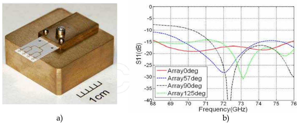
Fig. 15. a) Photograph of a four-element linear array prototype integrated with a microstrip-to-waveguide transition. b) Measured reflection coefficients for all arrays Radiation patterns and gain were measured in an anechoic chamber in CSIRO at 71.5 GHz, 72 GHz and 72.5 GHz. The radiation patterns were measured using a linearly polarized horn antenna at the transmitter. The simulated and measured co- and cross-polar radiation patterns of the array with the main beam in the broadside direction are shown in Fig. 16. Similar agreement between the simulated and measured results was achieved for the other three arrays and also at the other two frequencies.
