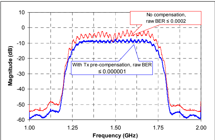
Fig. 24. Received signal at the output of A/D converter and measured BER for pre-compensated and un-compensated pseudo-random 8PSK symbols transmitted at 1.5 Gbps
