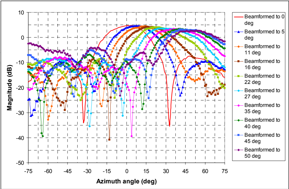
Fig. 21. Measured E-plane co-polar patterns for the array beam formed to a selection of positive azimuth angles
