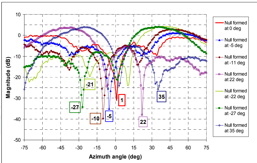
Fig. 20. Measured E-plane co-polar patterns for the array beam formed to cancel the main beam (form a null) at selected azimuth angle Labels appended to each pattern show actual measured null positions. Experimental results were in a very close agreement with analytical estimates ( \approx 1 degree). The array was steered to a selection of other positive and negative azimuth angles and E-plane antenna patterns were measured at each of the selected angles. The theoretical phase weights were applied to the null calibration reference settings to steer the beam to the non-zero azimuths. These
