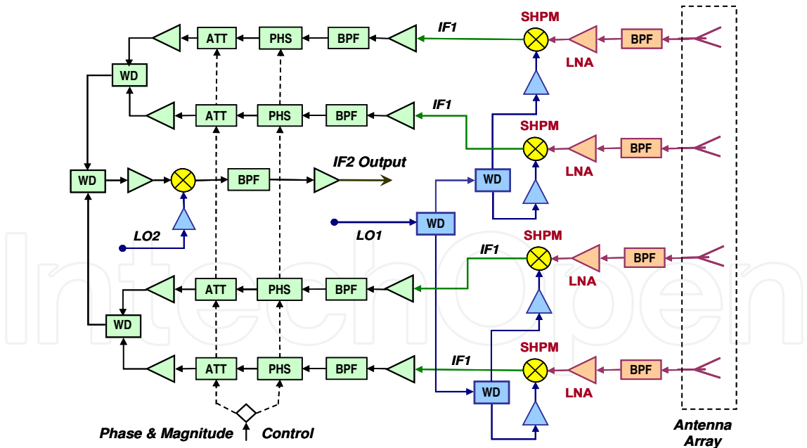
Fig. 6. Simplified schematic of the E-band steerable receive array configured for analogue beam-forming The receive IF module (Rx IF) has been developed in two versions. In the digital beam forming configuration, each of the IF channels is connected to a digital beam former that replaces the de-modulator. For the analogue beam forming configuration all IF outputs are combined before de-modulation as shown in Fig. 6 where BPF, LNA, SHPM, WD, PHS and
