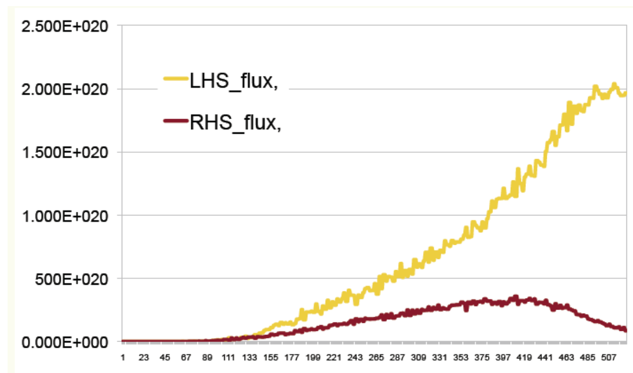
Fig. 6. Time evolution of inwards (LHS) and outwards (RHS) particle fluxes (in arbitrary units) as functions of time, estimated on the grid.
