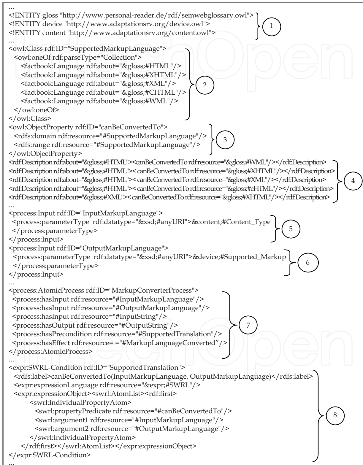
Fig. 23. OWL-S specification skeleton of a MLTS profile
