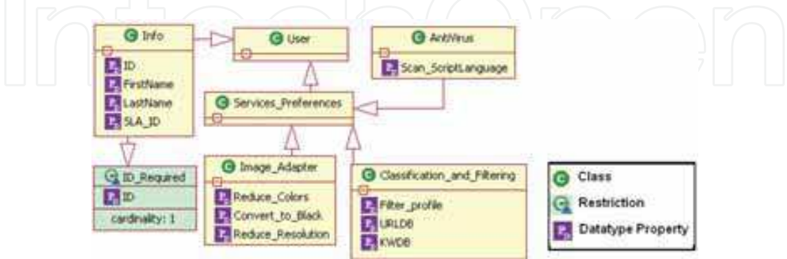
Fig. 17. Ontology model for a user profile
