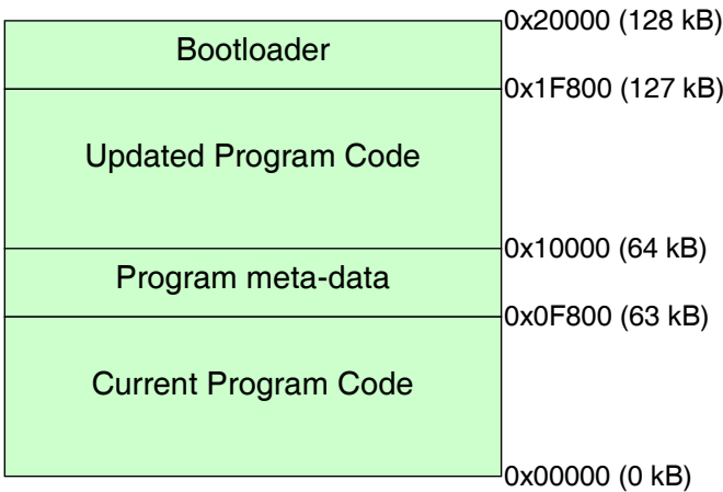
Fig. 5. ATmega128 program memory structure (byte addresses)
