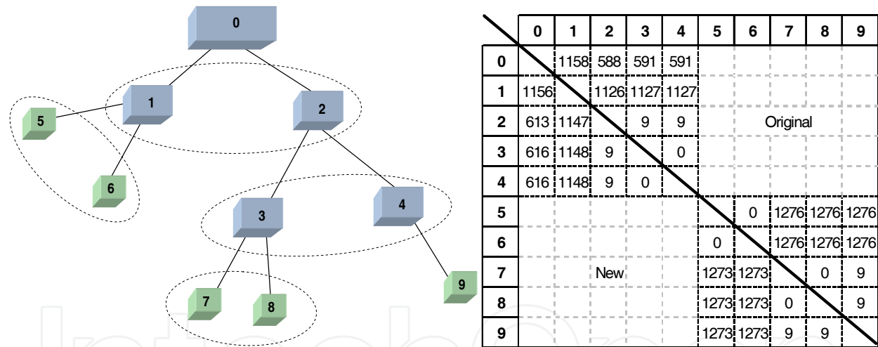
Fig. 9. Heterogeneous WSN topology and node application conversion costs
