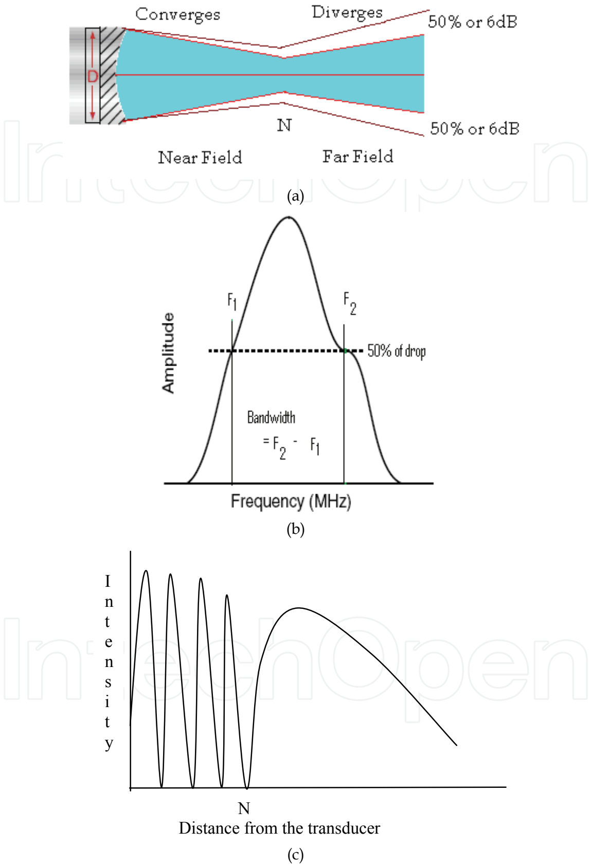
Fig. 2. (a) sound field of transducer, (b) amplitude versus frequency of UW, (c) intensity of UW versus axial distance from transducer.
