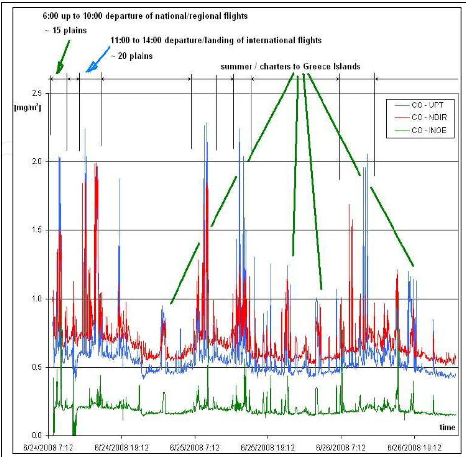
Fig. 15. CO measurements and airplanes traffic.
