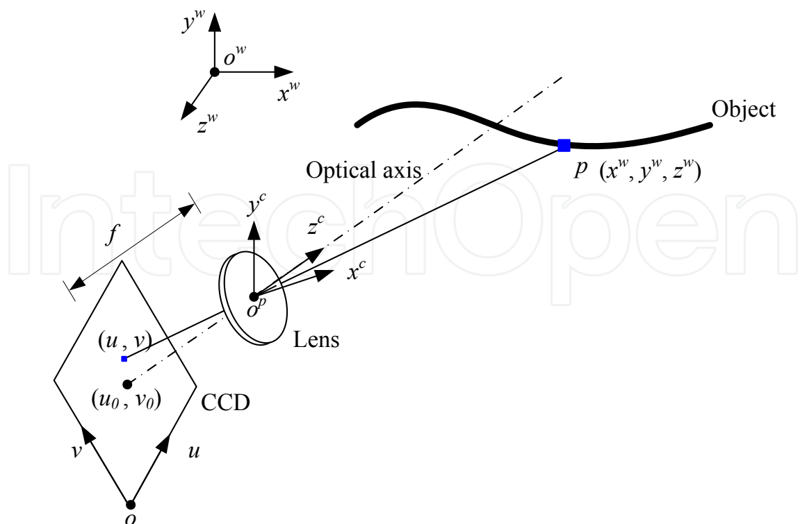
Fig. 3. Pinhole camera model. The camera model is to describe that an arbitrary point in 3-D space under its own coordinate system is transformed to the camera lens coordinate system, and finally 3-D coordinates in lens coordinate system are projected onto a 2-D imaging space.
