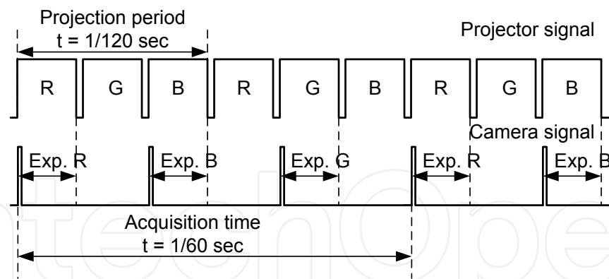
Fig. 7. System timing chart.
