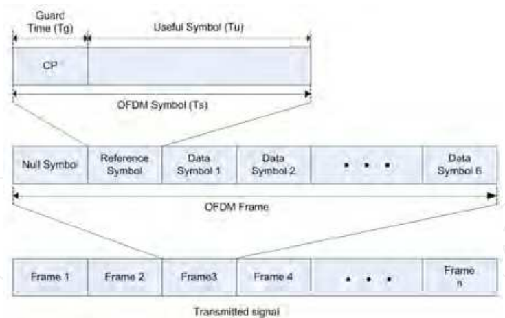
Fig. 2. OFDM frame structure
