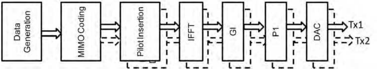
Fig. 12. Block diagram of the transmitter signal processing
