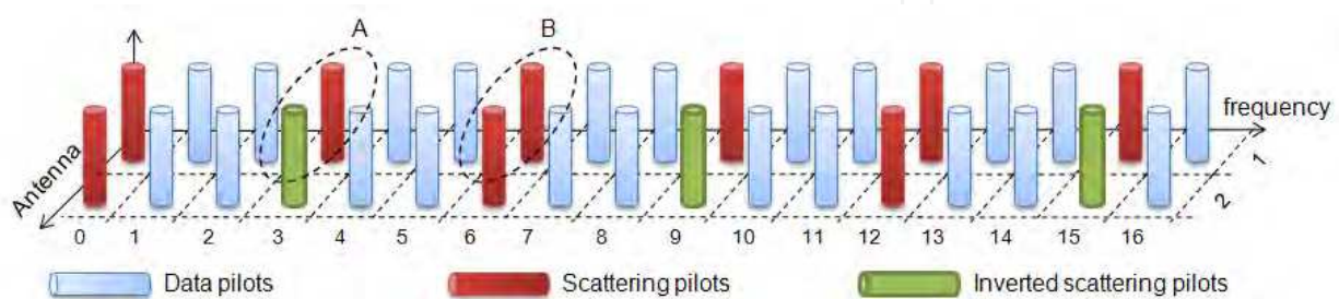
Fig. 17. Scattered pilots association for antennas 1 and 2
