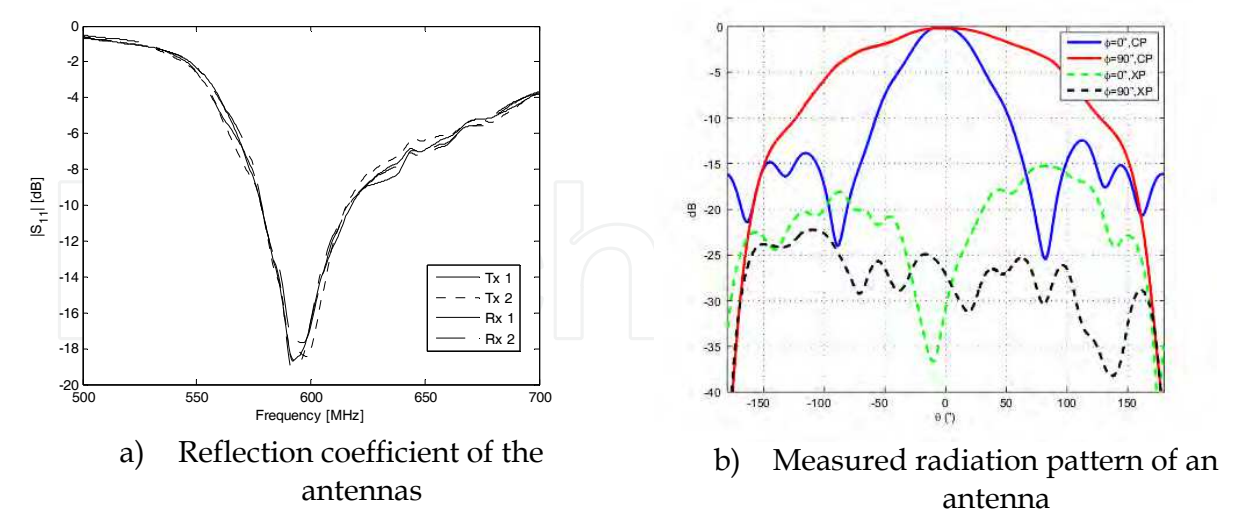
Fig. 18. Antenna performances
