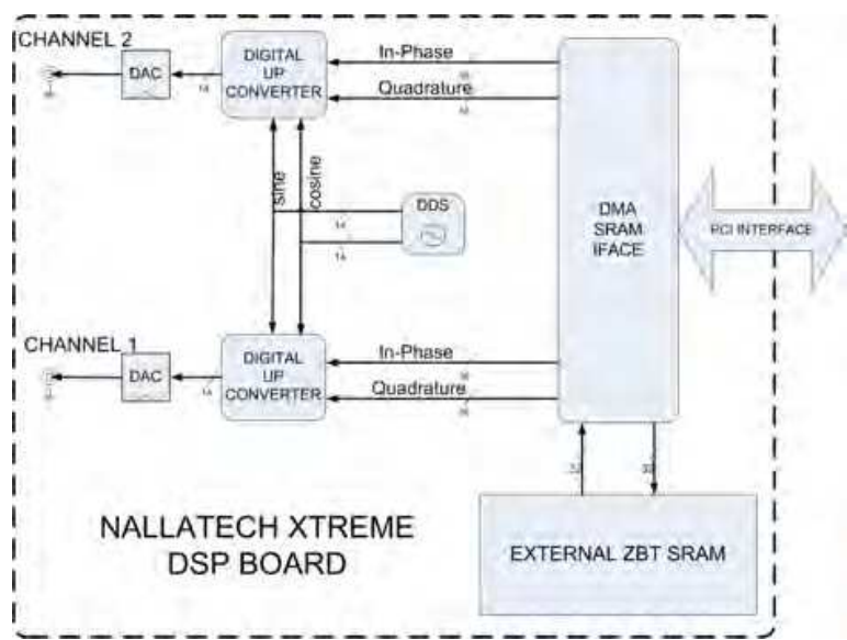
Fig. 13. Architecture of SDR transmitter
