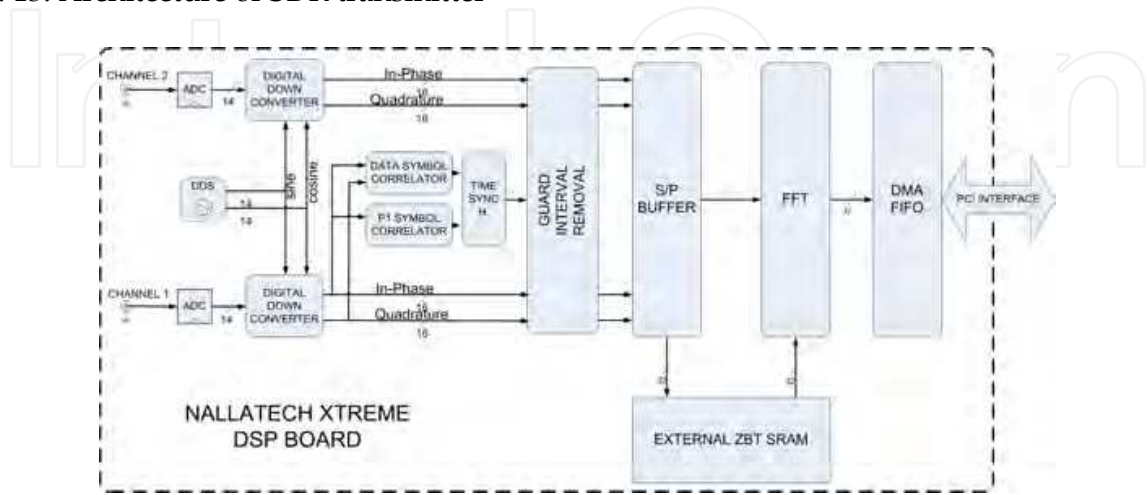
Fig. 14. Architecture of SDR receiver
