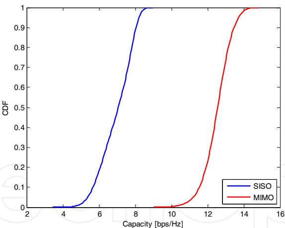
Fig. 21. Comparison of CDF of capacity with 1x1 and 2x2 in outdoor LoS case with polarization diversity
