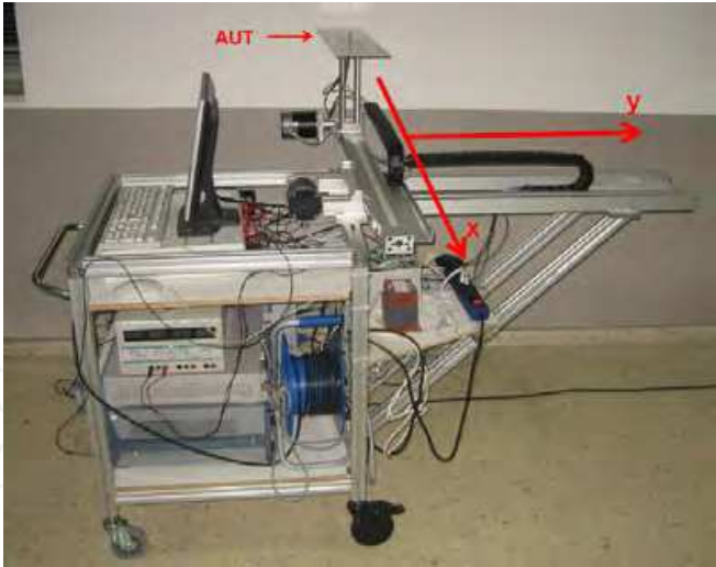
b)Receiver
