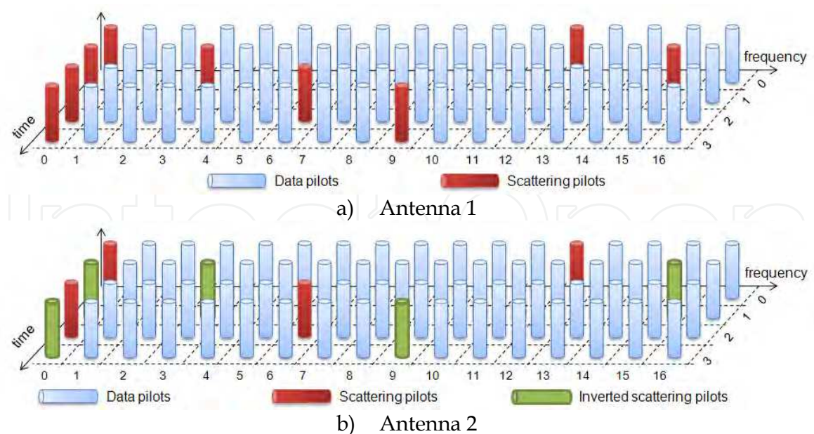
Fig. 16. Scattered pilots distribution
