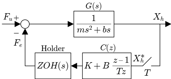
Fig. 2. Discrete haptic model.
