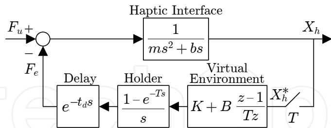
Fig. 4. Linear simplified model of a haptic system.
