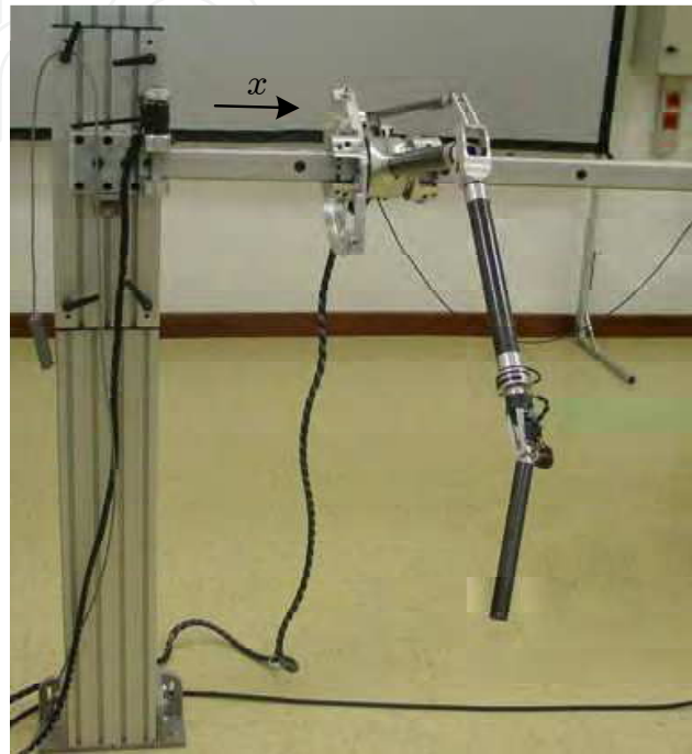
Fig. 7. LHfAM haptic interface.
