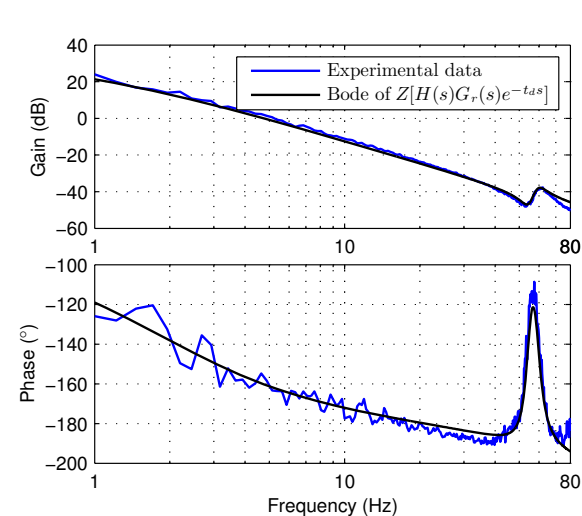
Fig. 14. Experimental (blue line) and theoretical (black line) Bode diagrams for the PHANToM.
