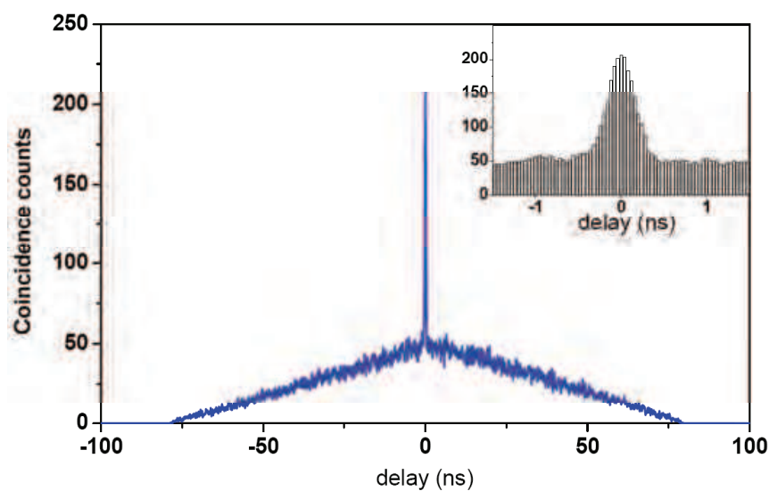
Fig. 12. Time-correlation histogram between counterpropagating photons.
