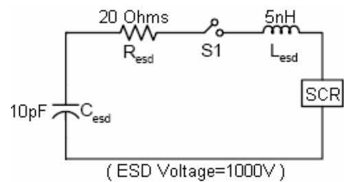
Fig. 15. Equivalent circuit of CDM Model
