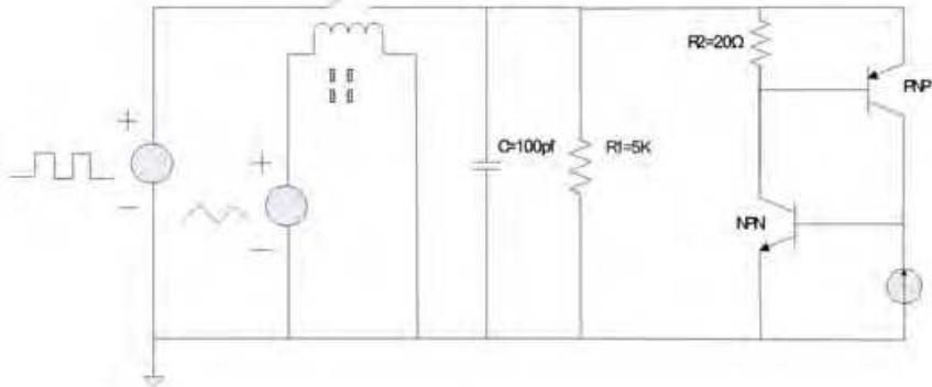
Fig. 31. ESD voltage pulse generation circuit and equivalent schematic of SCR
