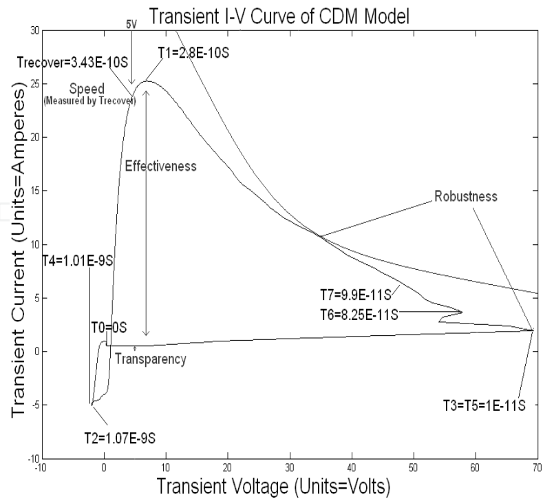
Fig. 23. Ransient I(t) versus transient V(t) of SCR-based ESD protection device
