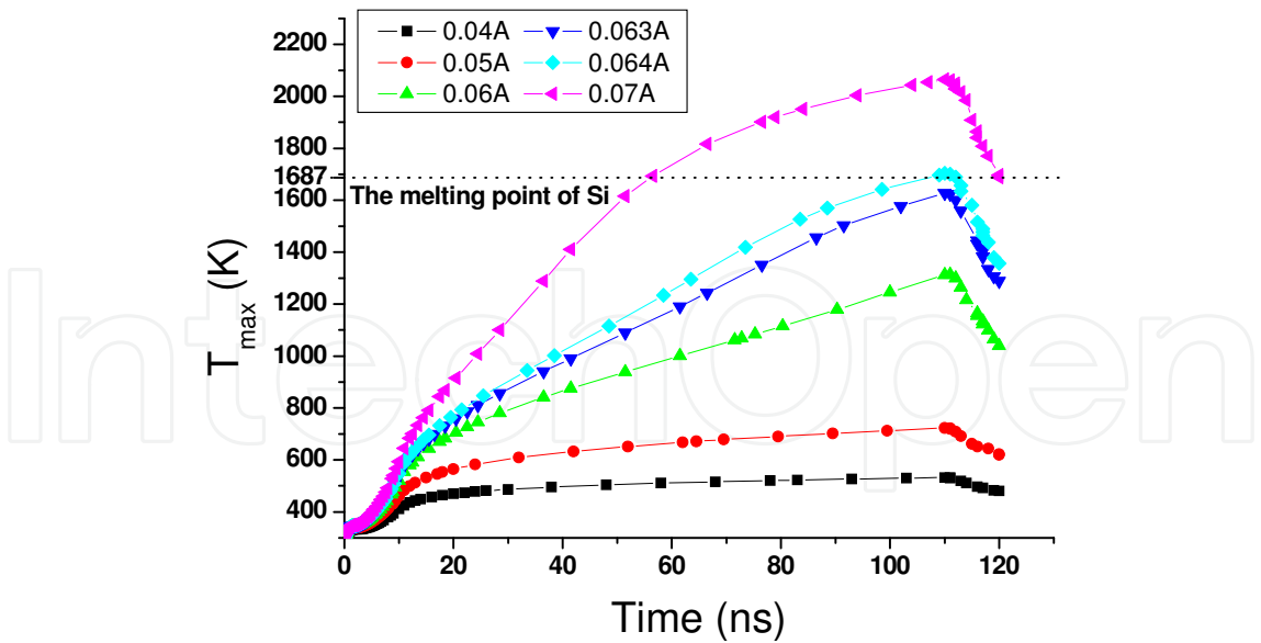
Fig. 14. Maximum temperature in the structure vs. time curves when series of current pulses are imposed on the structure.
