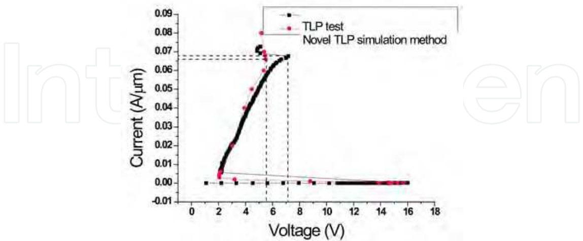
Fig. 13. I_{t2} obtained from novel TLP simulation and that from TLP test
