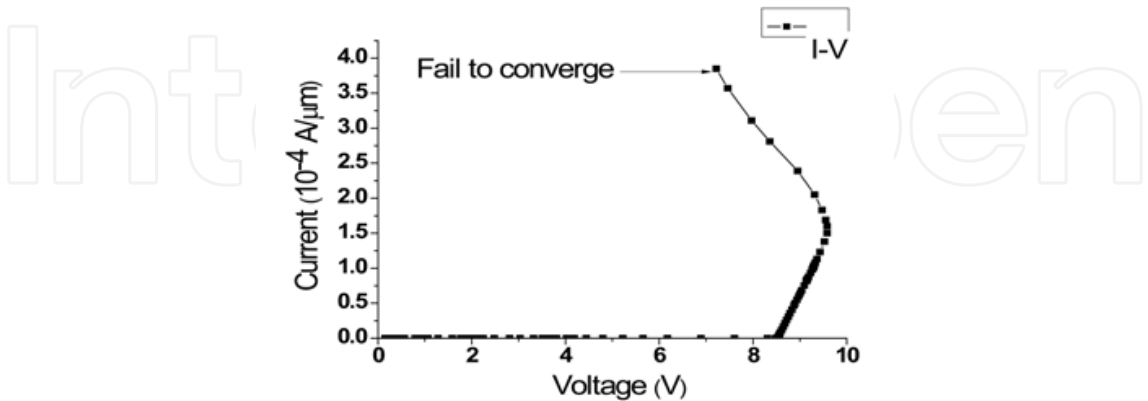
Fig. 6. Simulation fails to converge after the snapback happens
