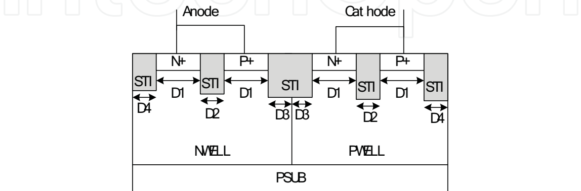
Fig. 7. A cross section of LSCR
