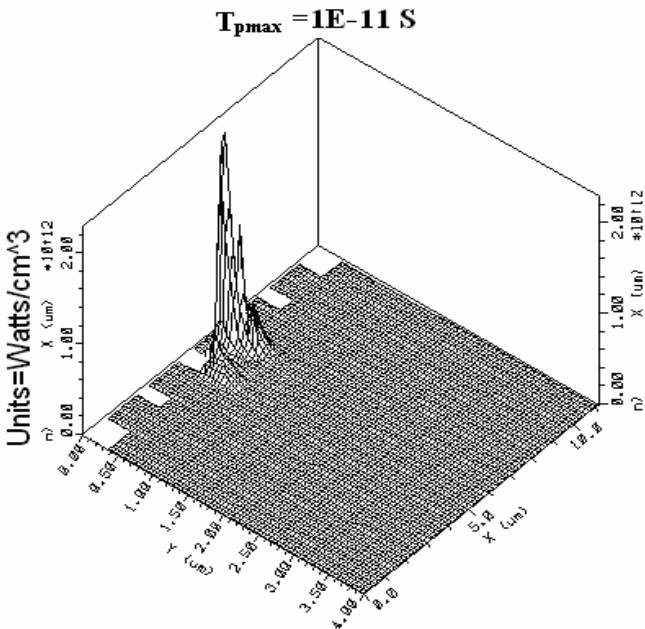
Fig. 21. The power distribution when the power comes to its peak
