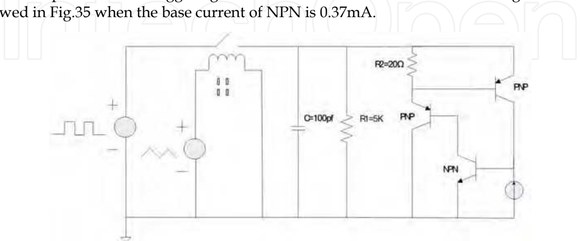
Fig. 33. ESD voltage pulse generation circuit and equivalent schematic of Darlington SCR
