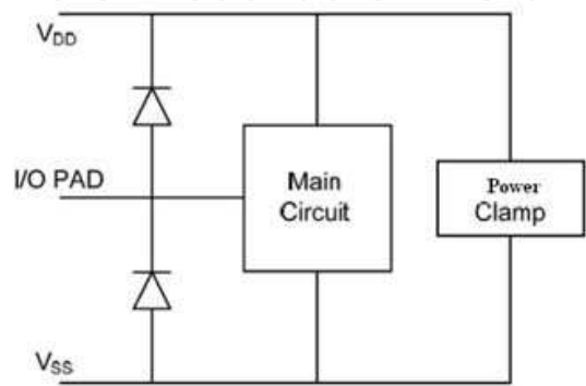
Fig. 24. Rail-based ESD protection scheme with power clamp
