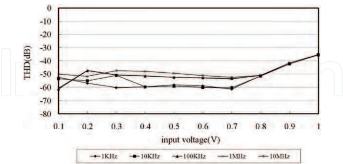
Fig. 12. Simulated THD for different input frequencies
