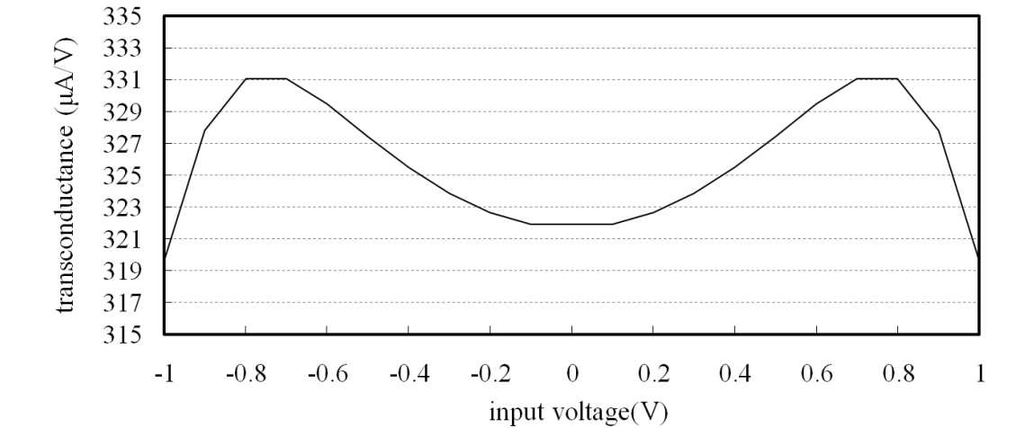
Fig. 10. The simulated transconductance at V_C=0.7V
