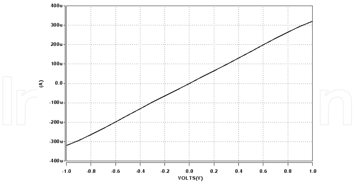
Fig. 9. V-I transfer characteristic
