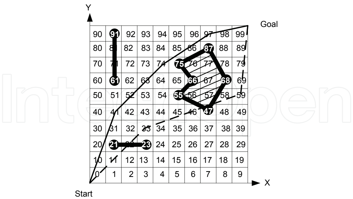
Fig. 5. Environment presented in form of occupancy grid. Numbers denote different nodes. Bold lines: obstacles; solid lines: feasible path; dashed line: unfeasible path.
