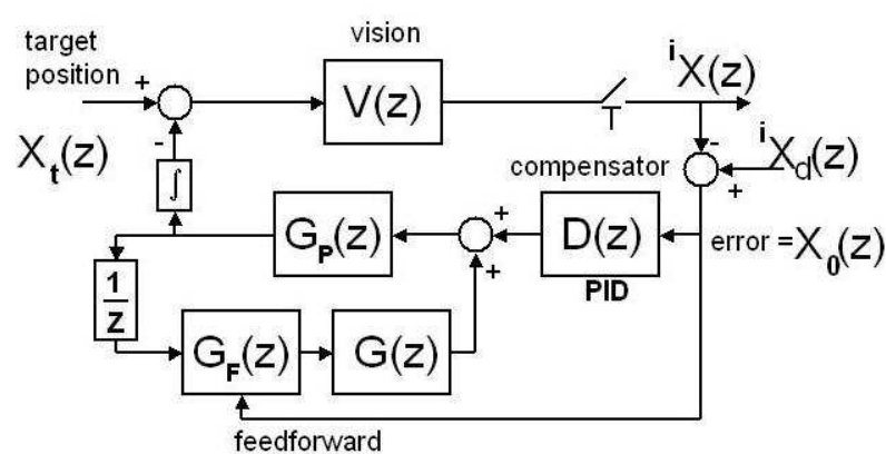
Fig. 7. Feedforward controller with a feedback compensation as it was implemented
