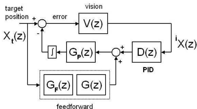
Fig. 6. Feedforward controller with a feedback compensation.
