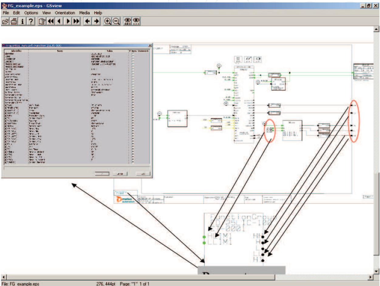
Fig. 14. Function Group example: parameters, implementation and symbol.
