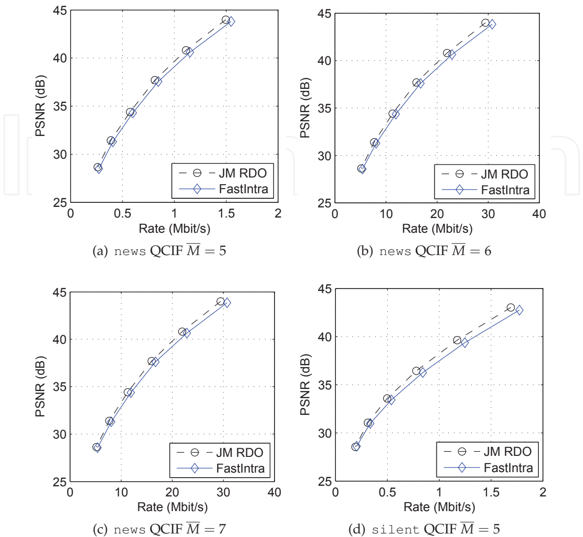
Fig. 8. PSNR vs. rate for only Intra coded sequences with different target number \overline{M} of candidates (Intra4x4 mode only).
