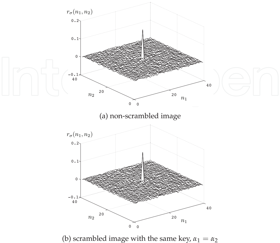
Fig. 7. Estimation of translation using DCT-SPC: (a) is the DCT-SPC surface between the non-scrambled images, and (b) is the DCT-SPC surface between the sign phase-scrambled images. (a) and (b) are identical, and an acute peak appears at the location expressing the translational displacement.
