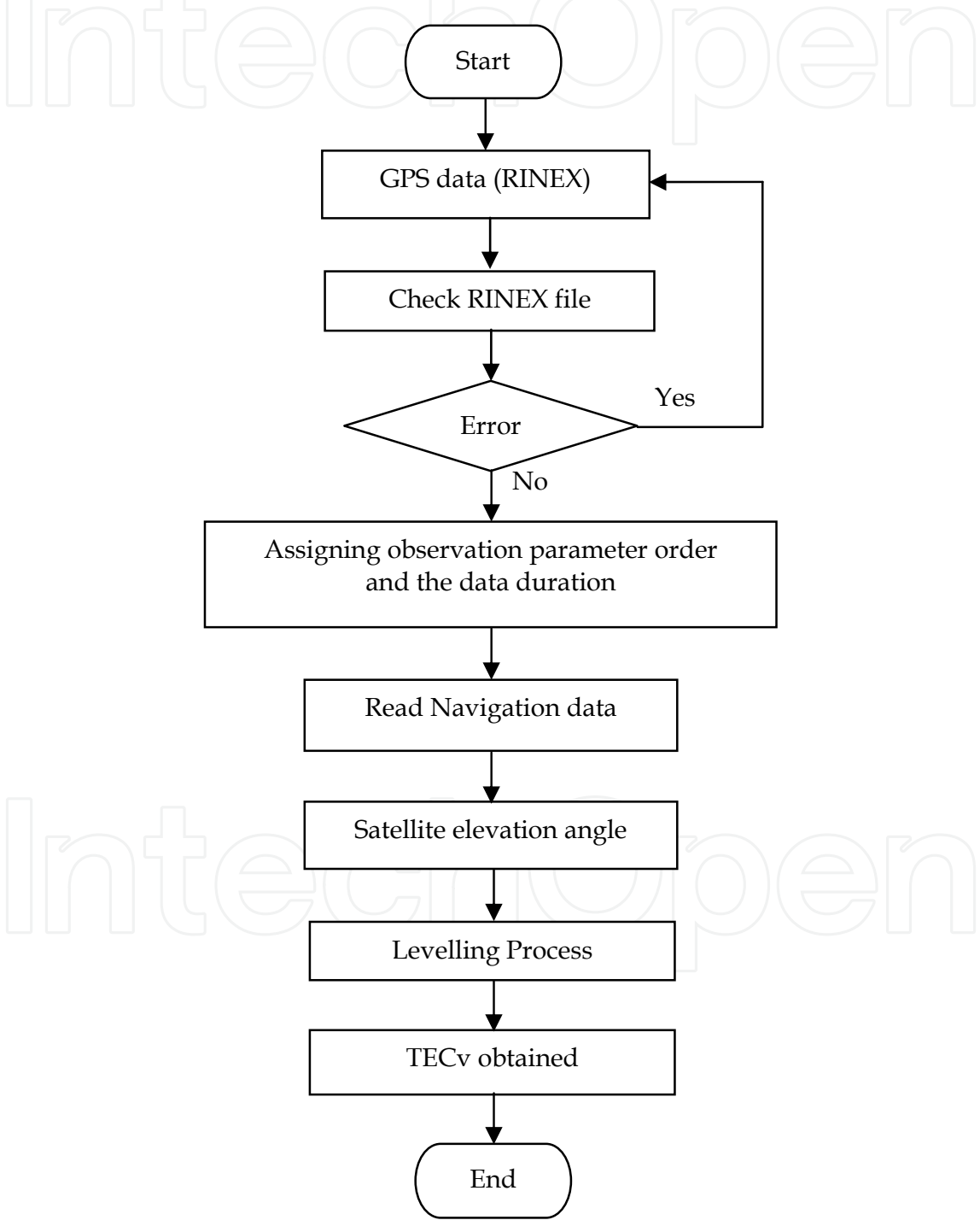
Fig. 3. Flowchart of TEC processing
