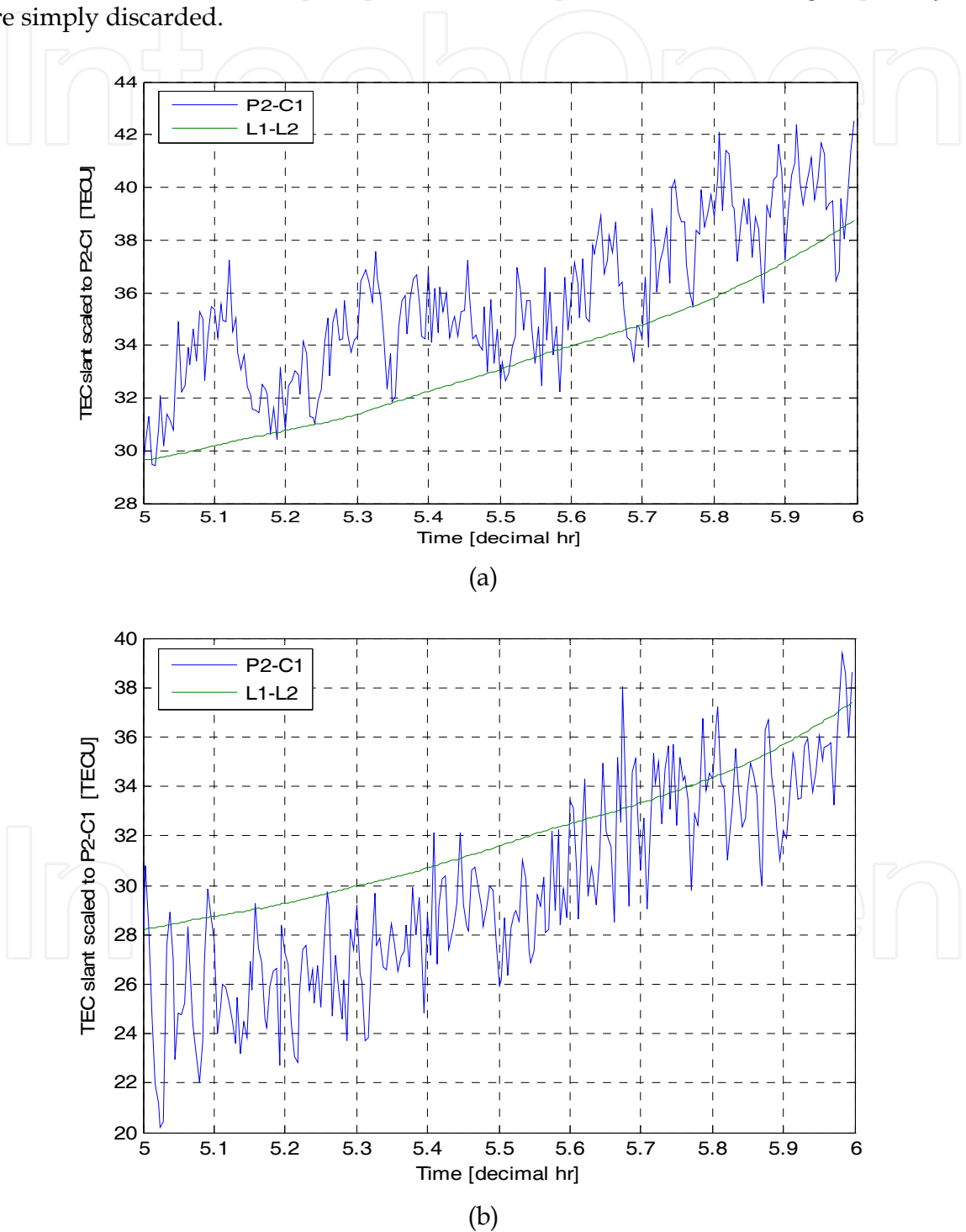
Fig. 10. (a) TEC slant scale to (P2- C1) TECU for PRN 23, 5:00-6:00 UT (KTPK station) (b) TEC slant scale to (P2- C1) TECU for PRN 23, 5:00-6:00 UT (UTMJ station)
