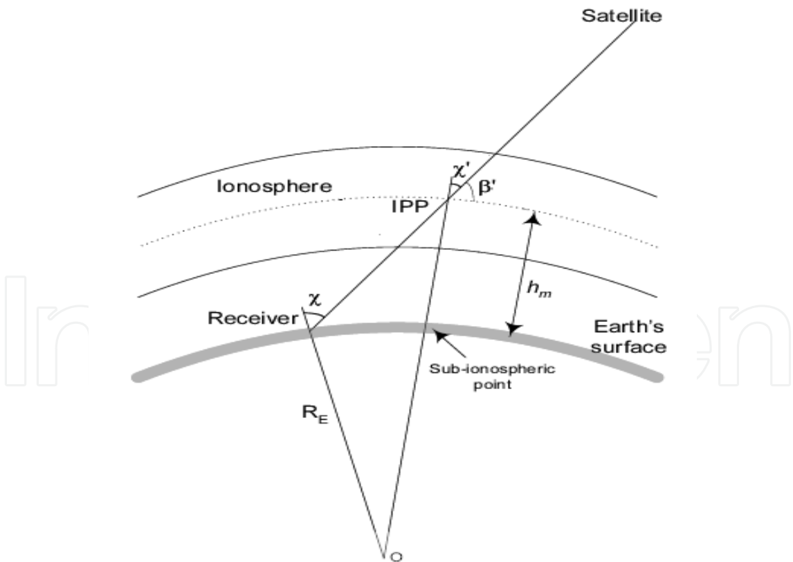
Fig. 4. Ionospheric Single Model (SLM) Source: Schaer 1996
