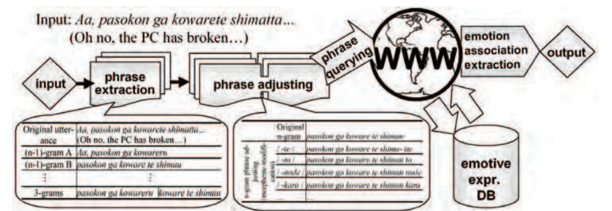
Fig. 5. Flow chart of the Web mining technique
