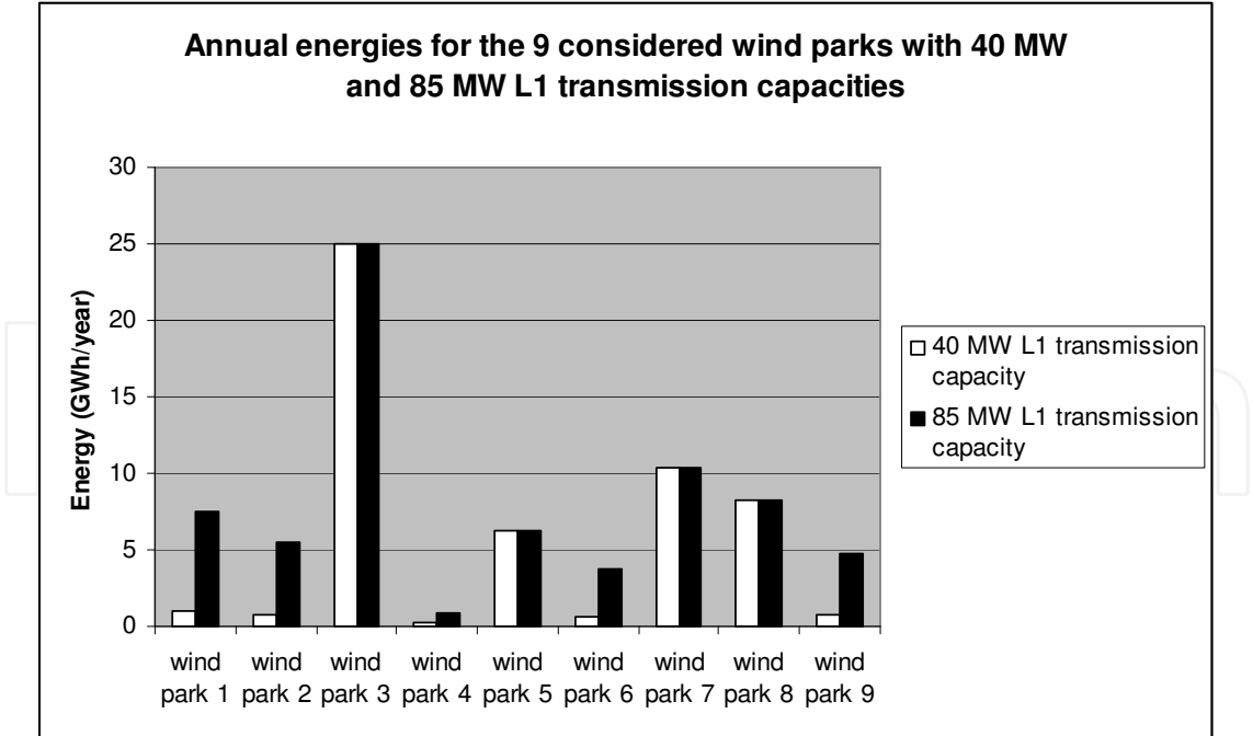
Fig. 9. Annual energy (GWh/year) for the 9 considered wind parks with 40 MW (white) and 85 MW (black) L1 transmission capacities
