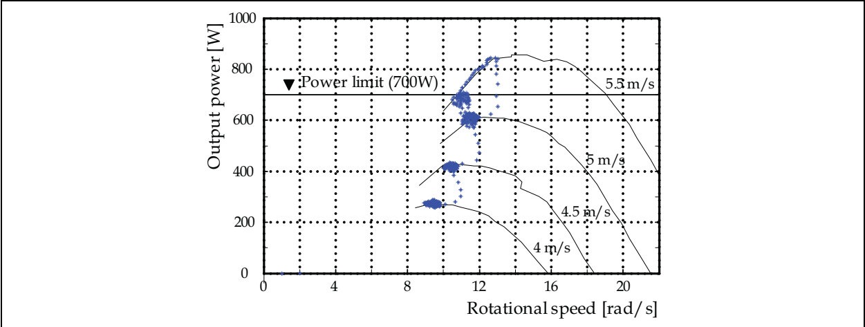
Fig. 18. Control trajectory of searching-based MPPT searching algorithm
