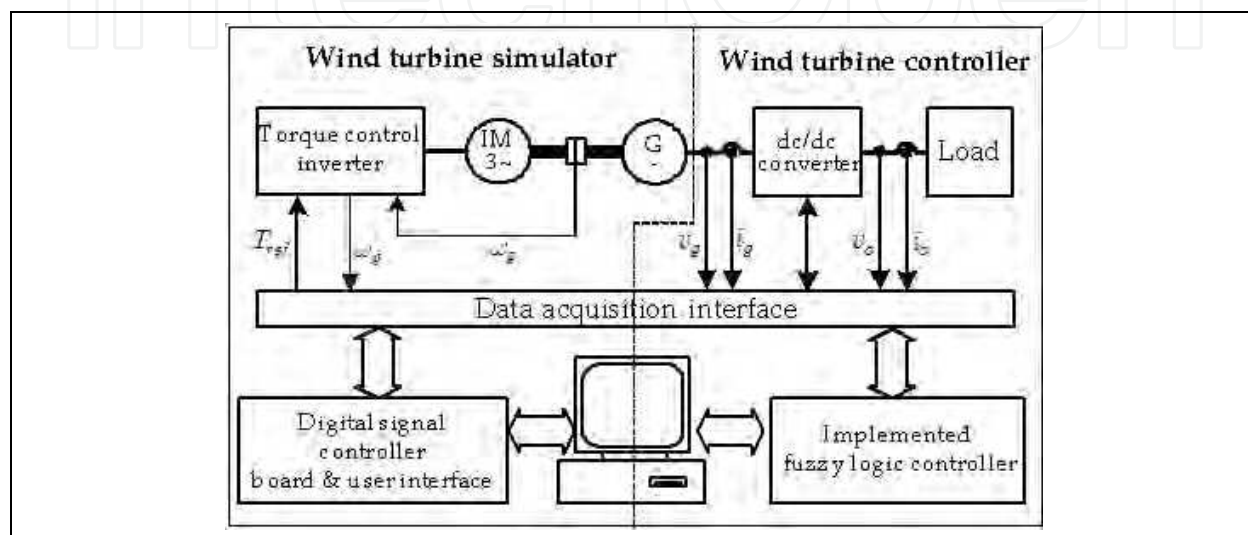
Fig. 16. Test system
