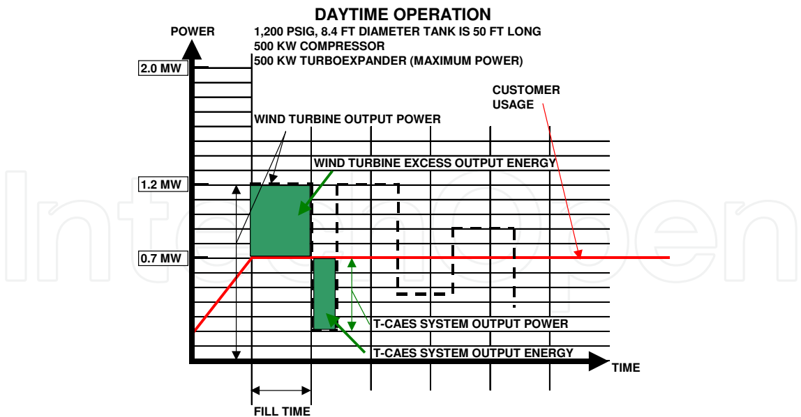
Fig. 14. Overall principal of T-CAES system (Enis Windgen)
