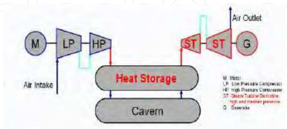
Fig. 11. Advanced Adiabatic CAES Concept (Alstom Power)
