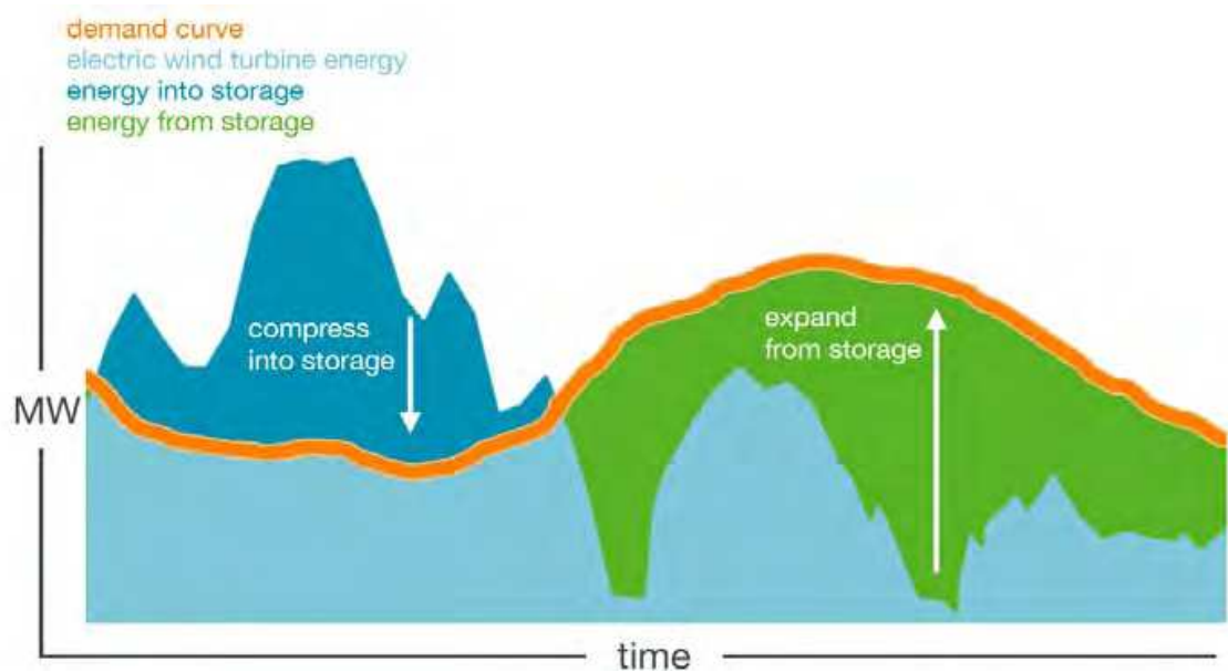
Fig. 6. Meeting the demand curve with stored wind energy (General Compression) cycle. The Huntorf, Germany and the McIntosh CAES plant compressors are driven by the Generator which operates as a motor during the compression cycle. This limits the flexibility of the plant which today allows compression power to be designed with multiple units to accommodate different rated compression units to balance the wind variability. This optimization allows a larger range of options for different geographical regions with wind variances.
