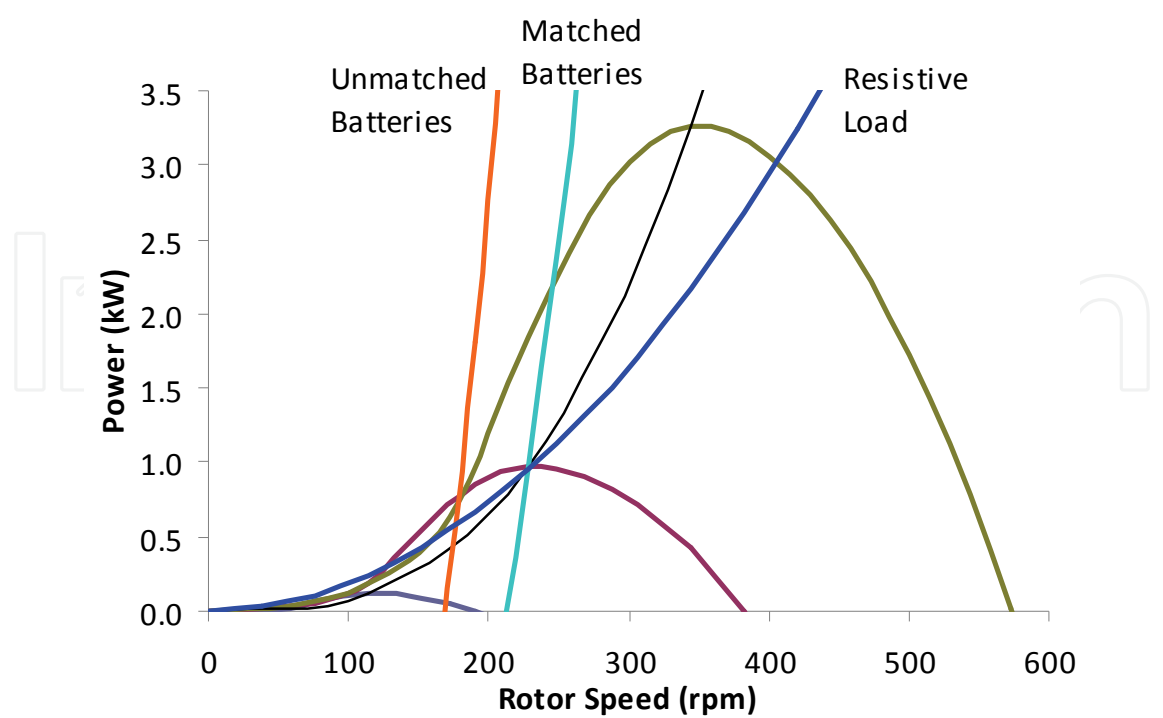
Fig. 27. Power of the turbine and loads versus turbine speed
