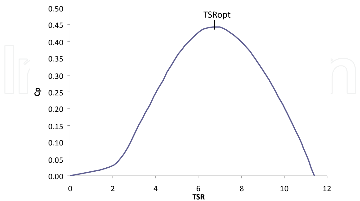
Fig. 2. Coefficient of performance as a function of tip-speed-ratio for a wind turbine.
