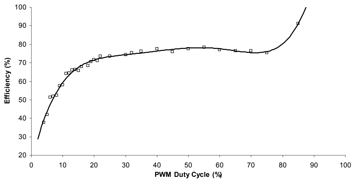
Fig. 23. Efficiency of the DC-DC converter versus duty cycle at constant load and PWM frequency Above 80% duty cycle the efficiency jumps to 90% because the OFF time of PWM is insufficient to drive the IGBT fully OFF. In this case the DC-DC converter begins to act as low impedance resistive link between the generator and the load.
