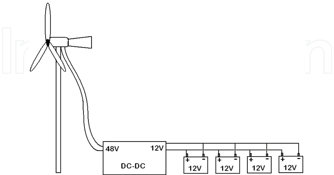
Fig. 9. Wind Turbine with DC-DC Step Down Converter charging batteries
