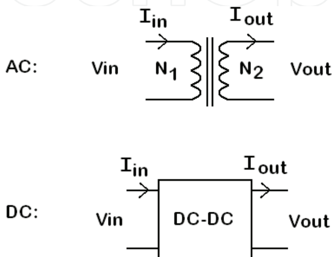
Fig. 5. AC and DC voltage/current converters
