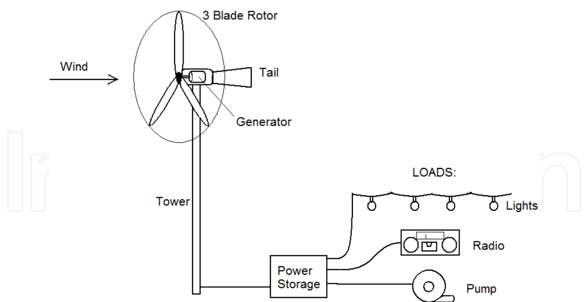
Fig. 1. Schematic diagram of a typical small wind turbine power system. common configuration is a 3-blade, horizontal axis wind turbine directly driving a 3-phase permanent magnet generator. The output power of a wind turbine is function of wind velocity cubed. It can be described mathematically by (1).
