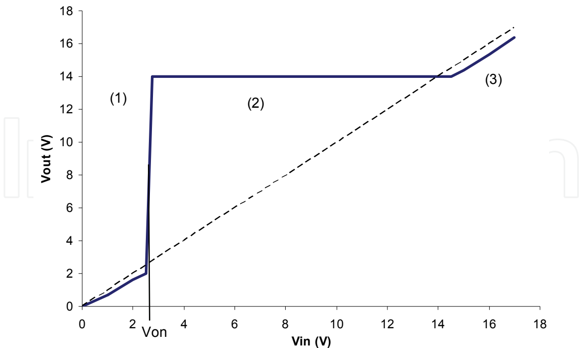
Fig. 8. DC-DC boost converter output voltage versus input voltage
