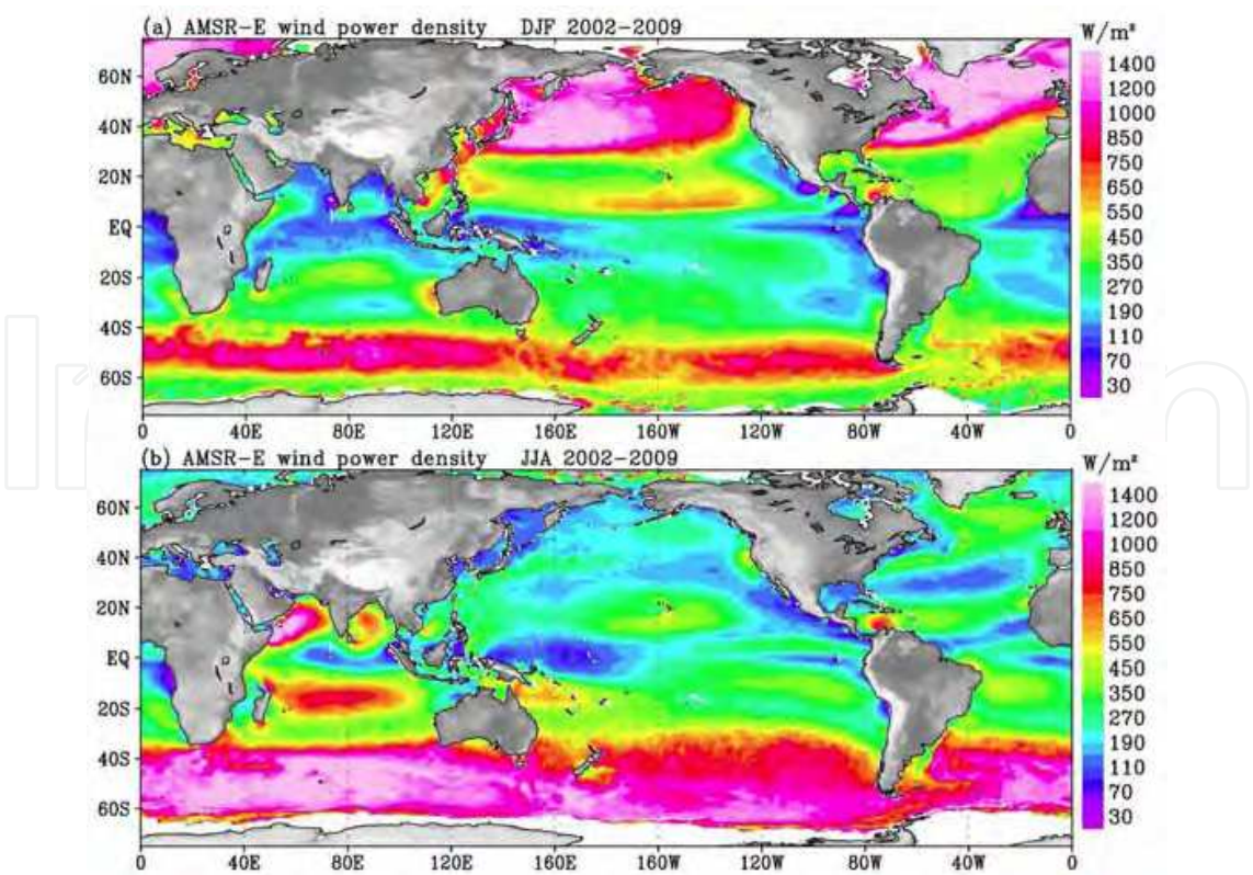
Fig. 3 Same as Fig. 2, but from AMSR-E.
