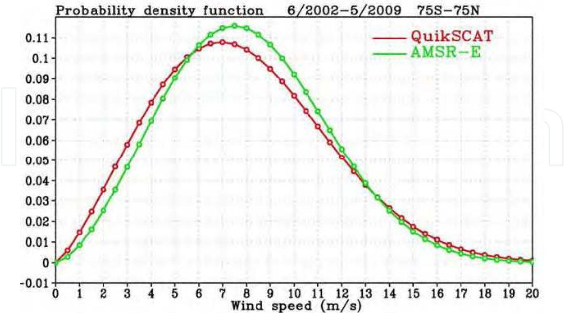
Fig. 1. Comparision of the probability density function of ocean surface wind speed from 7 years of QuikSCAT and AMSR-E measurements.
