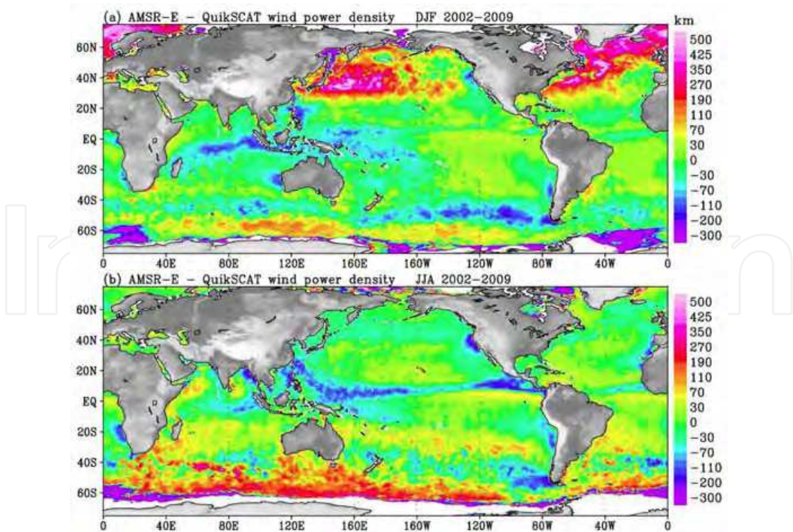
Fig. 4. Difference of wind power density between AMSR-E and QuikSCAT for (a) boreal winter and (b) boreal summer.
