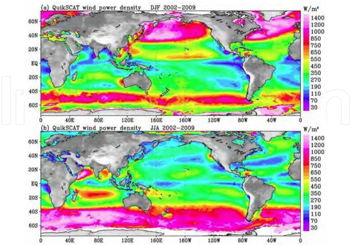
Fig. 2. Distribution of power density of ocean surface wind (10 m) from QuikSCAT for (a) boreal winter (December, January, and February) and (b) boreal summer (June, July, and August).
