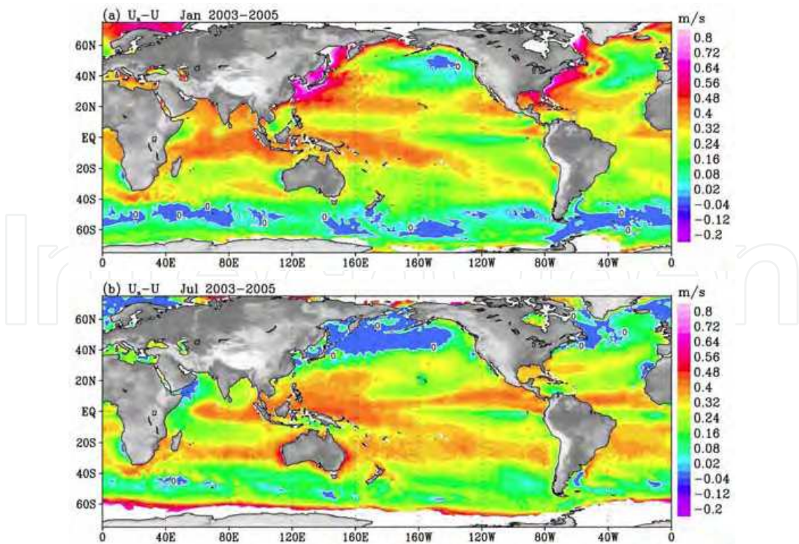
Fig. 7. Difference between equivalent neutral wind and actual wind at 10 m for (a) Januray and (b) July.
