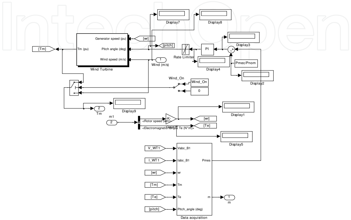
Fig. 7. Pitch controller block
