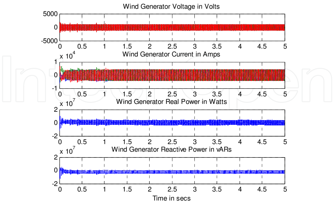
Fig. 12. Generator-side electrical outputs, normal operation
