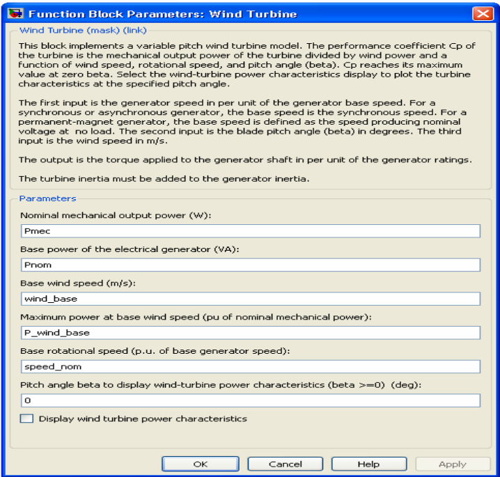
Fig. 8. Wind Turbine mask dialogue
