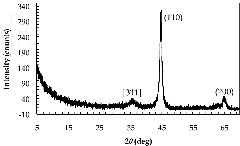
Fig. 4. XRD of 8.7 \pm 2.7 \text{ }\mu\text{m} long by 318 \pm 51 \text{ nm} diameter iron wires. The lattice planes for iron are indicated in ( ) brackets and those resulting from the oxide layer are indicated in [ ] brackets.
