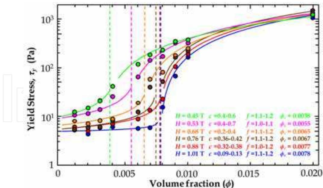
Fig. 9. The apparent yield stress ( \tau_y ) of on-state, cobalt-nanowire MR fluids as a function of nanowire volume fraction ( \phi ) for varying applied magnetic fields. The solid curves represent the best fit to expected power-law dependence given in Eq. 8 and 9. Data up to \phi = 0.06 was used in the analysis, but not shown for the sake of clarity near the critical point.
