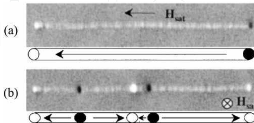
Fig. 9. Domain-imaging of a single 35 nm Co nanowire by magnetic force microscopy after saturation in a magnetic field applied (a) parallel and (b) perpendicular to wire axis (Reprinted with permission from [Ebels et al., 2000]. Copyright (2000) by the American Physical Society.). (For Co wires with aspect ratio of 10, the critical diameter is 140 nm.)
