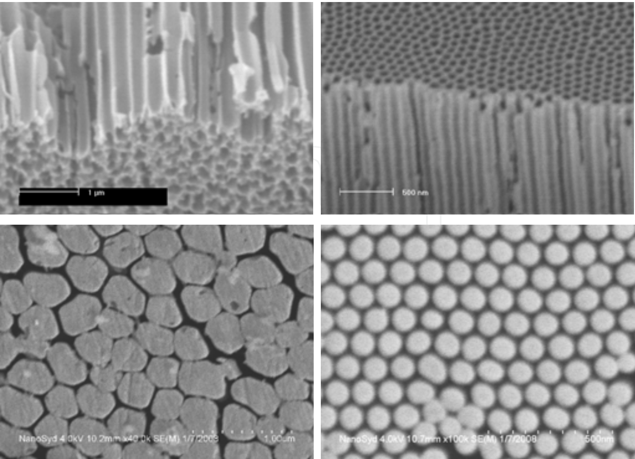
Fig. 3. Cross sectional view of (a) Anodisc™ AAO (quoted pore size 200 nm) and (b) doubleanodized AAO (0.3M oxalic acid, 40V). (c, d) Topographic view of the same templates upon pore filling and subsequent mechanical polishing (bright features correspond to metal nanowires; dark regions correspond to AAO pore walls).
