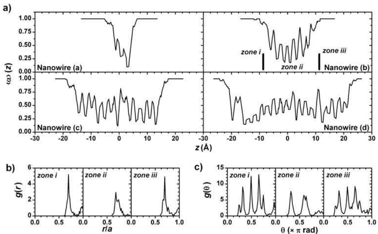
Fig. 10. a) Average \alpha -parameter \langle\alpha\rangle(z) along the Ni [110] simulated nanowire showed in Fig. 9 before breakage. Minimum values of \langle\alpha\rangle below 0.5 correspond to the position of pentagonal rings forming the icosahedral nanowire. b-c) Distance g(r) and radial g(\theta) distributions for the three marked region of the nanowire labelled as (b).
