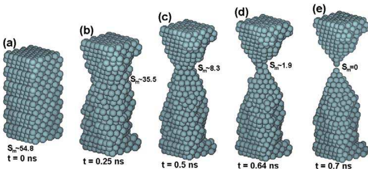
Fig. 1. Five different snapshots of a [111] Ni nanowire during stretching at T = 300 K from its initial parallelepiped shape. Each snapshot includes information on the simulation time and the minimum cross-section S_m at that time.
