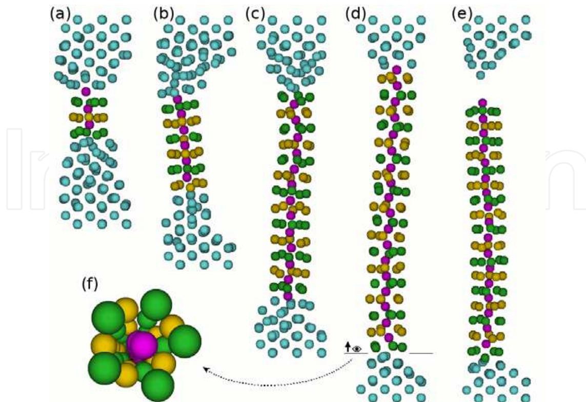
Fig. 9. (a-e) Formation, growth and breakage of an icosahedral nanowire from a small [110] Ni nanowire at T=550\text{K} ; (f) shows the cross-sectional perspective view as seen from the position indicate on (d). Colours are used to identified the -5-1-5-1- structure.
