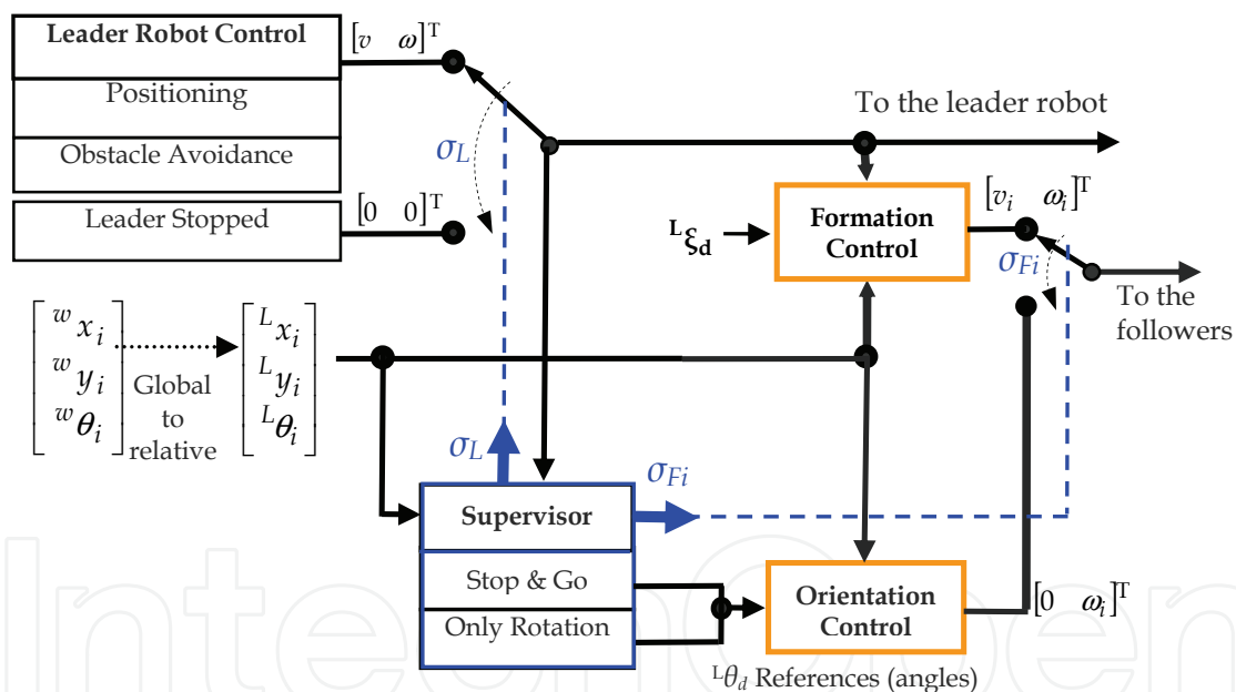
Figure 6. Hybrid formation control block diagram
