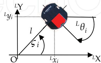
Figure 2. i -th follower in the leader coordinate system
