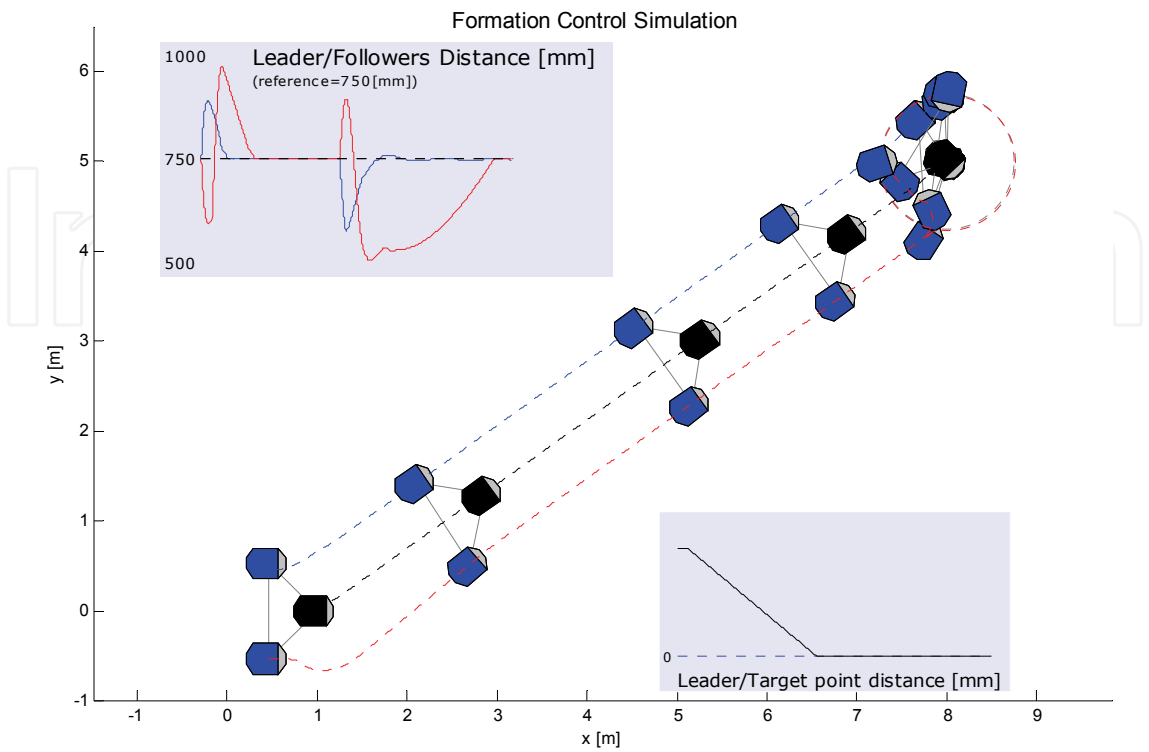
Figure 11. Formation control simulation
