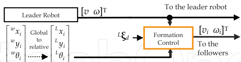
Figure 4. Formation control block diagram
