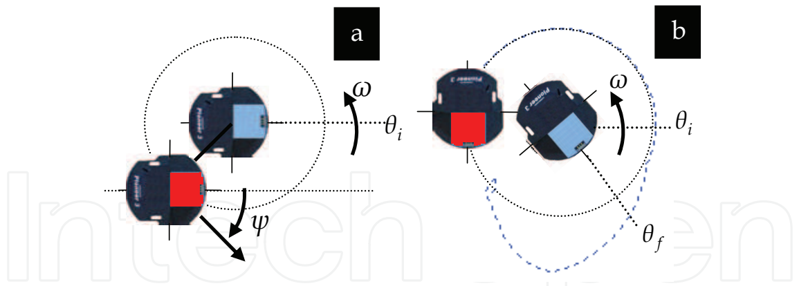
Figure 7. Formation control without orientation control for a leader (at the centre) and a follower: a) initial configuration; b) the path described by the follower (dotted line)
