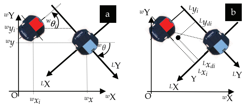
Figure 1. a) Reference systems: world (absolute) reference coordinate system ( O\ wX\ wY ), and a second coordinate system attached to the leader robot ( O\ LX\ LY ) where the desired positions for each of the followers are defined. b) i -th follower robot positioned at coordinates (Lx_i, Ly_i) on the leader Cartesian reference where the reference position is given by (Lx_{di}, Ly_{di})
