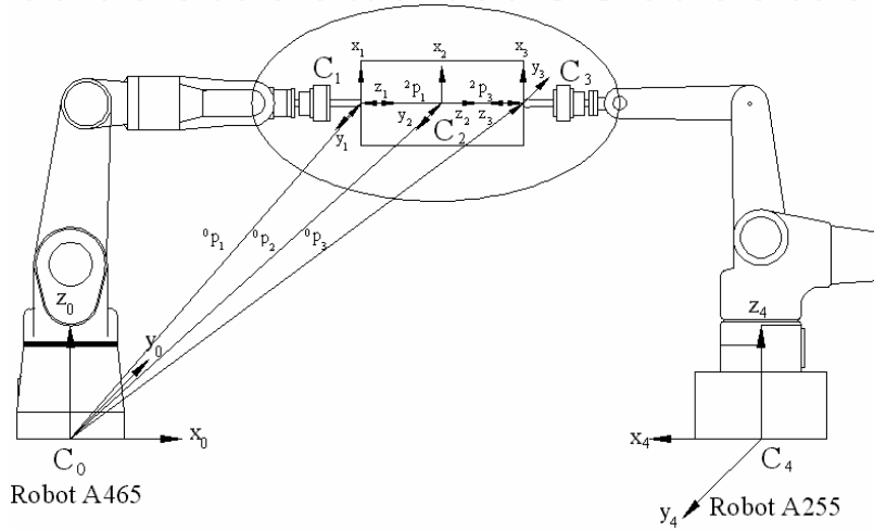
Fig. 2. Schematic diagram of robots holding an object.
