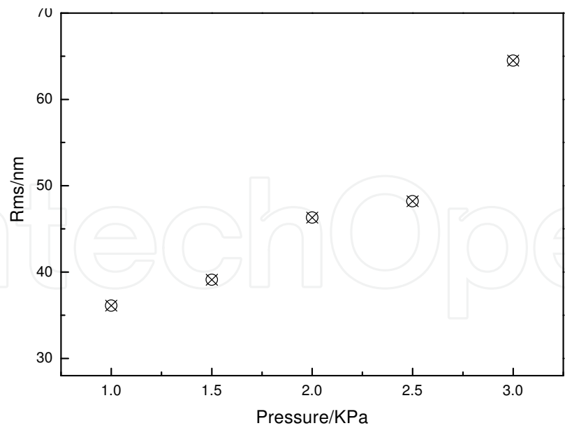
Fig. 4. RMS changes of nano-crystalline diamond films under different deposition pressure
