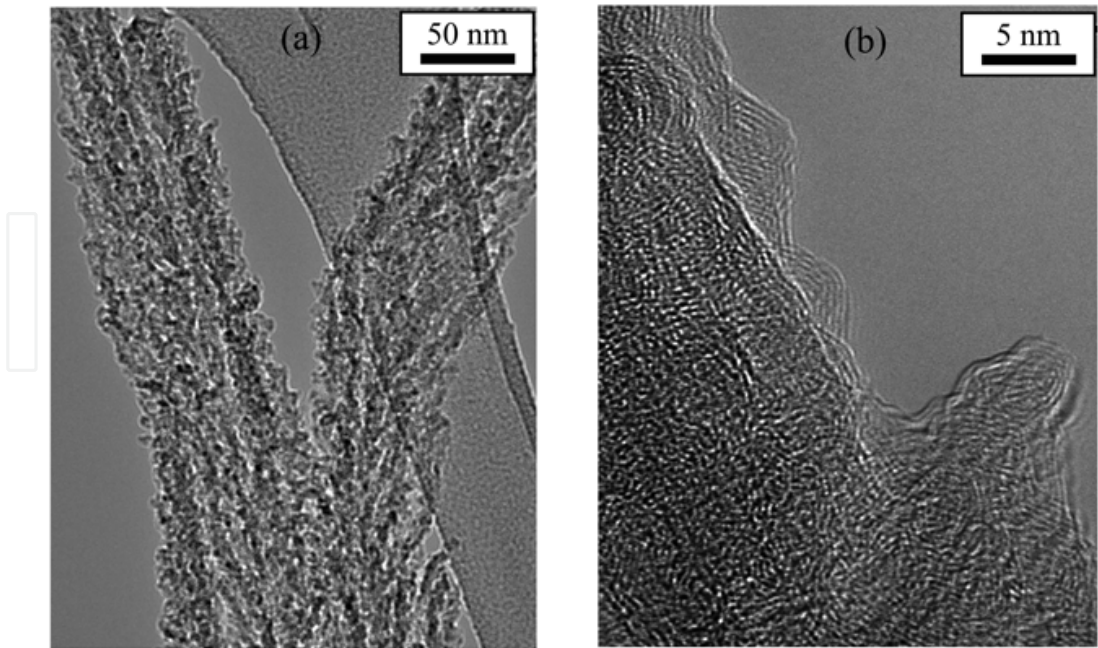
Fig. 8. TEM images of CNFs grown on the glass substrates at an O 2 /CO ratio of 7/1000. (a) Low-magnification TEM image of two bundling CNFs; (b) high-magnification TEM image of the CNF surface.
