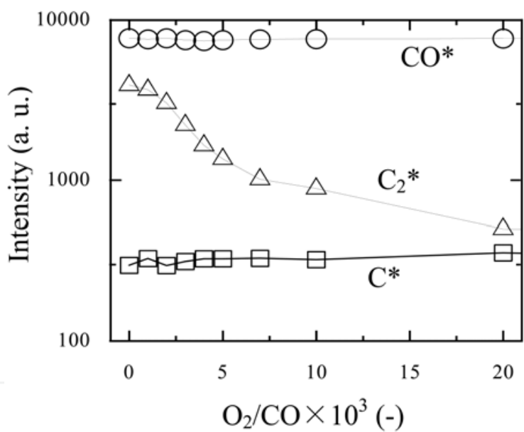
Fig. 11. Emission intensity of CO^* , C_2^* , and C^* as a function of O_2/CO ratio rates decrease drastically with increasing additional oxygen fraction and show a good correlation between them. In general, the change in the precursor density and the increase in the etching ability are thought to be the reasons why CNFs disappears as the amount of oxygen increases. However, as shown in the previous study, it cannot be thought that an increase in the etching ability is the reason for the disappearance of the CNFs in this case. When the small amount of hydrogen was added to the CO/Ar plasma, the CNFs disappear but the carbon deposits are not removed. As for the change in the spectrum, it is only C_2 molecules that the emission intensity shows a substantial change when the amount of hydrogen increases (Mori & Suzuki, 2008). In other words, even if the etching ability is low, the suppression of C_2 molecule formation results in the disappearance of fibrous structure. The carbon etching ability of hydrogen is much lower than that of oxygen (Mucha et al.,
