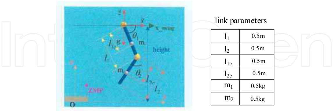
Fig. 13. The link model.
