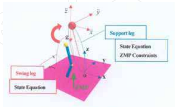
Fig. 12. Swing leg Formulation Model.
