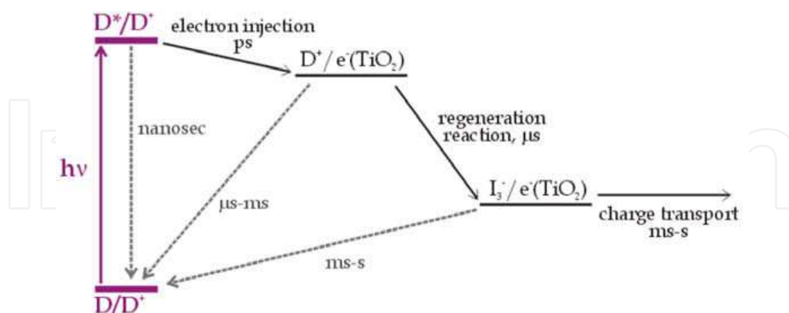
Fig. 2. Kinetics and competitive processes involved in the conversion of light to electric power in DSSC.
