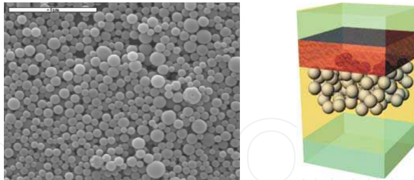
Fig. 4. Left: Scanning electron microscopy image of a slab made of polydisperse sub-micrometer \text{TiO}_2 particles that can be used as diffuse scattering layer in DSSC. Right: Scheme representing a DSSC with a “double layer” architecture.
