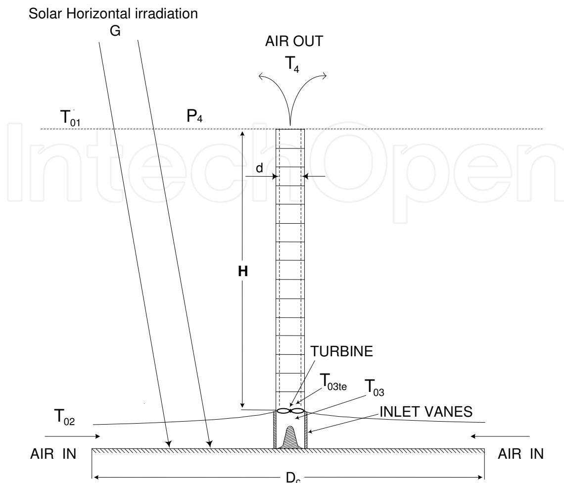
Fig. 4. Schematic diagram of the SAEF in operation
