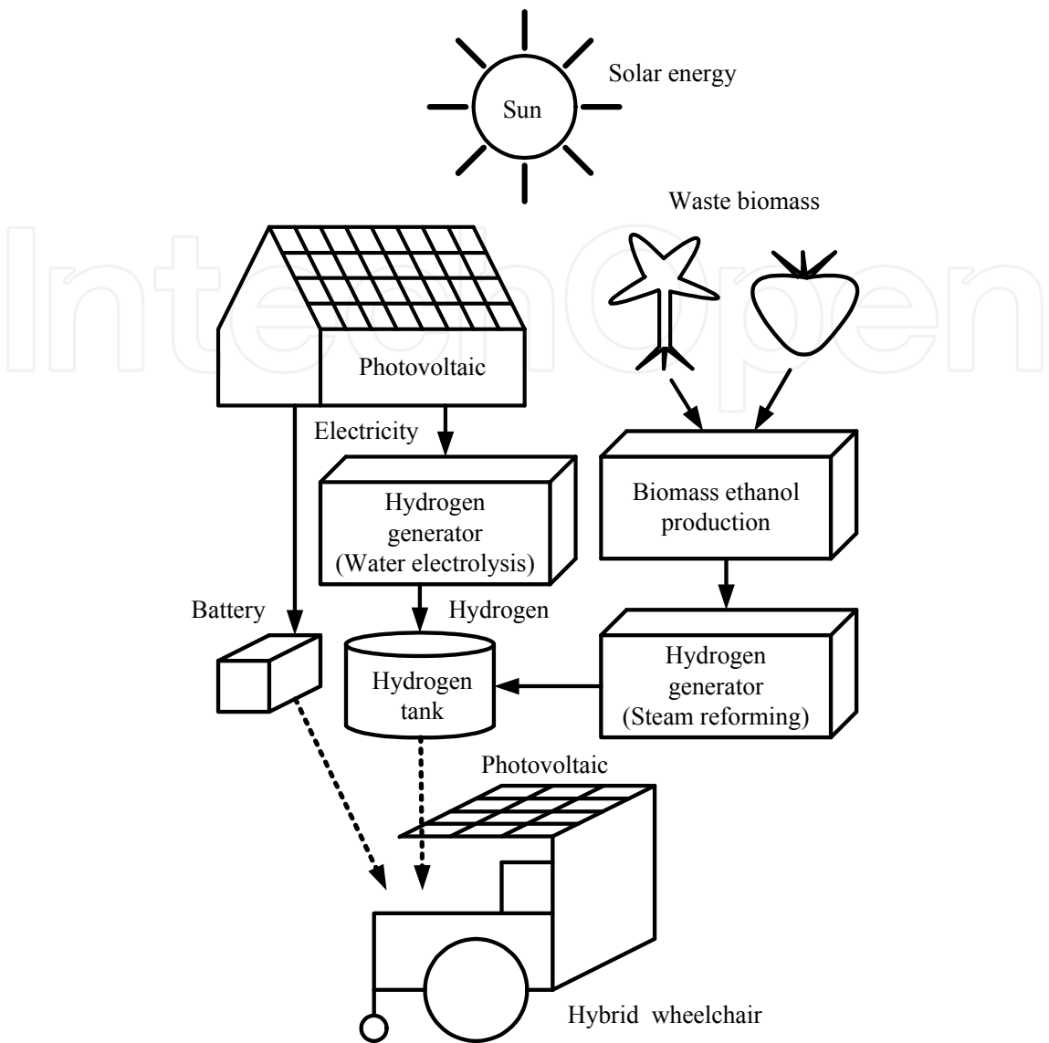
Fig. 2. Schematic explanation of energy flow
