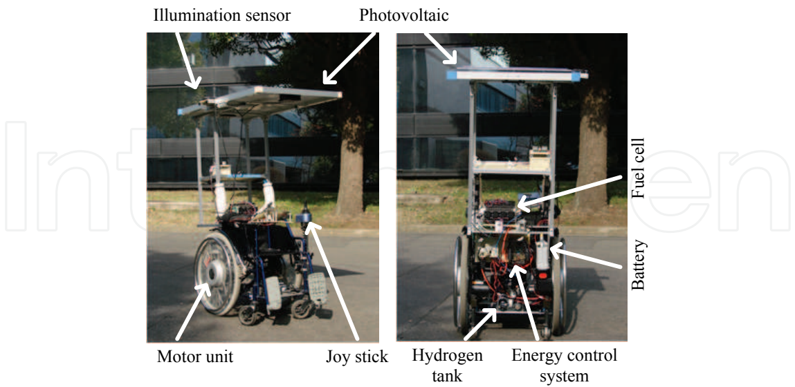
Fig. 4. Fabricated robotic wheelchair with photovoltaic and fuel cell
