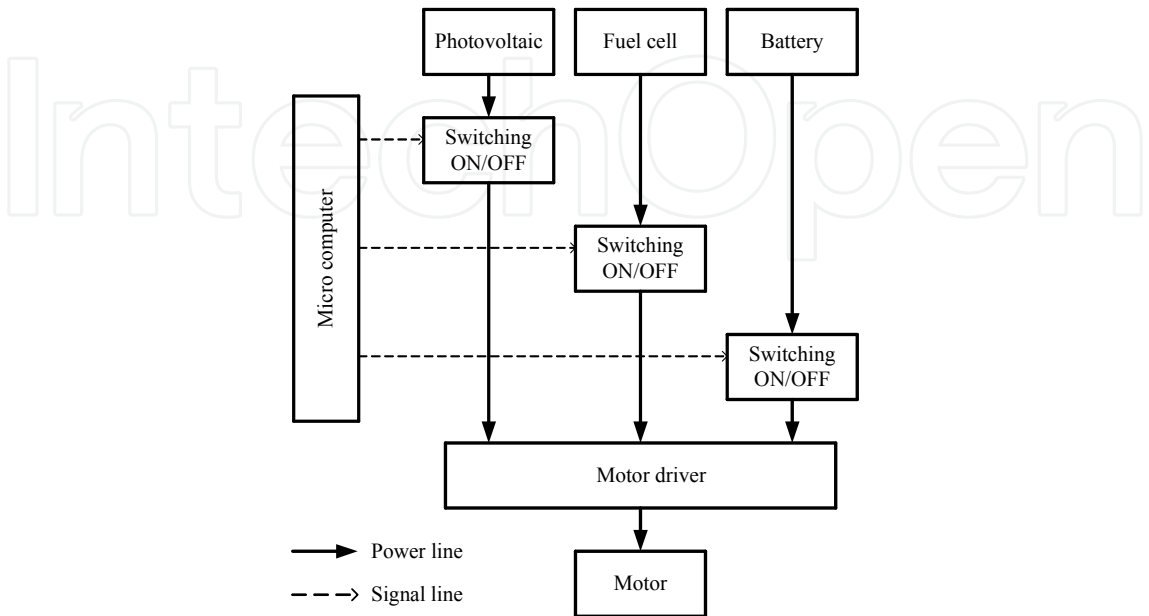
Fig. 7. Concept of energy control system
