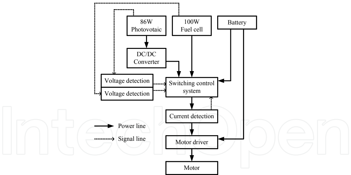
Fig. 8. Detailed energy control architecture
