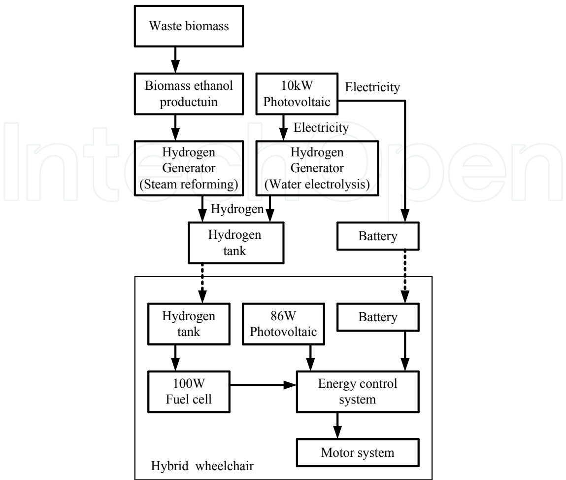
Fig. 3. Block diagram of energy flow
