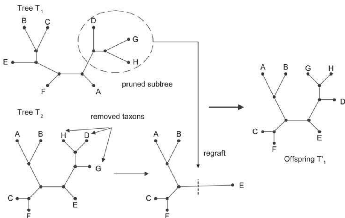
Fig. 2. Example of the crossover operator.
